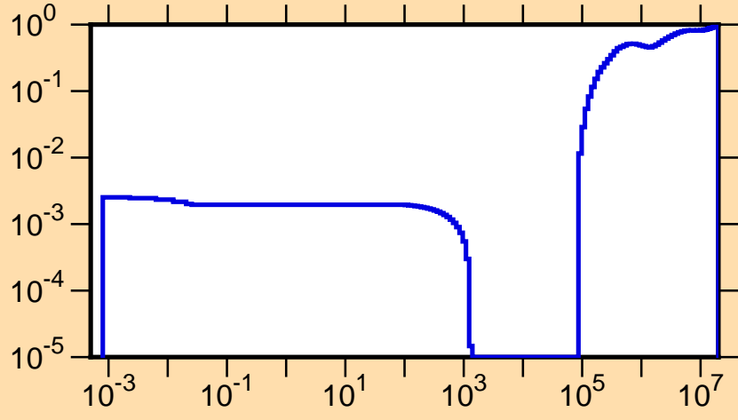
\mu vs. E for ^{262}\text{Md}(\text{mt251})
