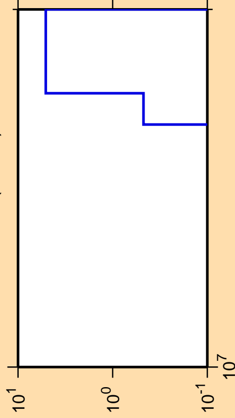
\Delta\sigma/\sigma vs. E for ^{262}\text{Md}(n,3n\alpha)
