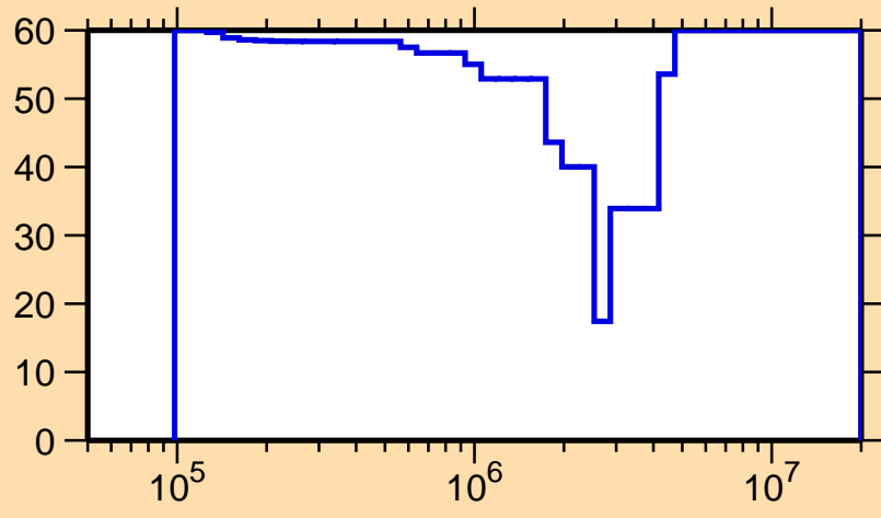
\Delta\sigma/\sigma vs. E for ^{262}\text{Md}(n,n\text{cont.})
