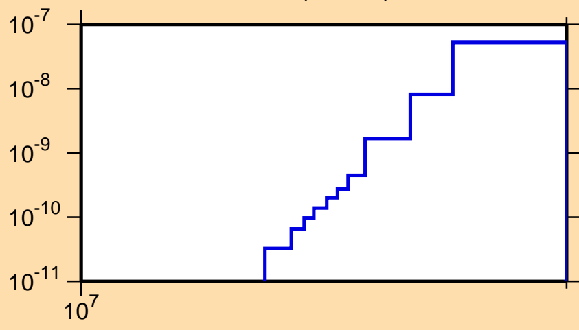
\sigma vs. E for ^{262}\text{Md}(n,2n\alpha)
