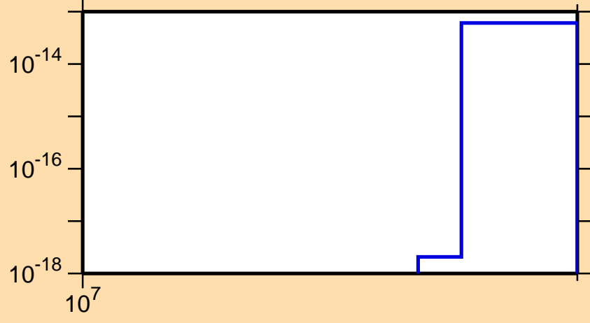
\sigma vs. E for ^{262}\text{Md} (mt 11)
