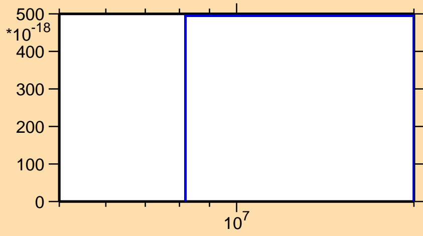
\sigma vs. E for ^{262}\text{Md}(\text{mt } 11)
