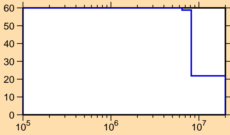
\Delta\sigma/\sigma vs. E for ^{262}\text{Md}(n,n_1)
