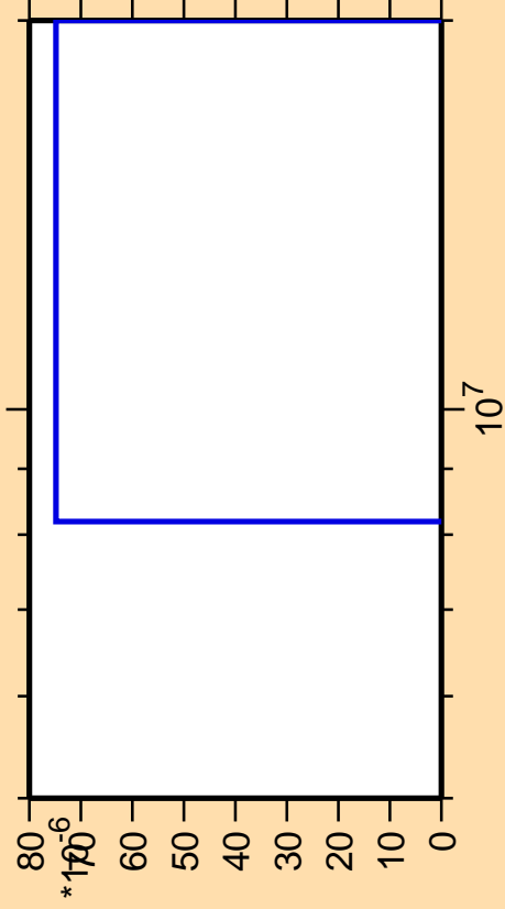
\Delta\sigma/\sigma vs. E for ^{262}\text{Md}(\text{mt } 11)
