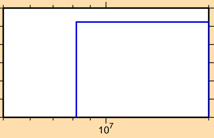
\sigma vs. E for ^{262}\text{Md}(n,nt)
