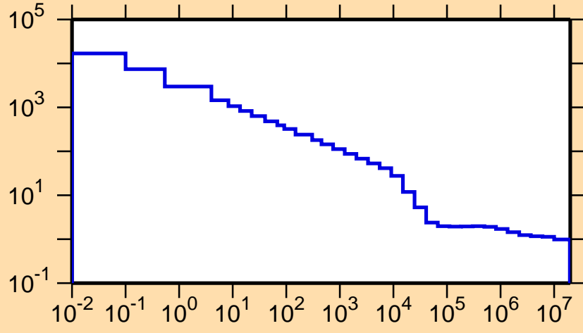
\sigma vs. E for ^{22}\text{Mg}(n,\text{nonel.})
