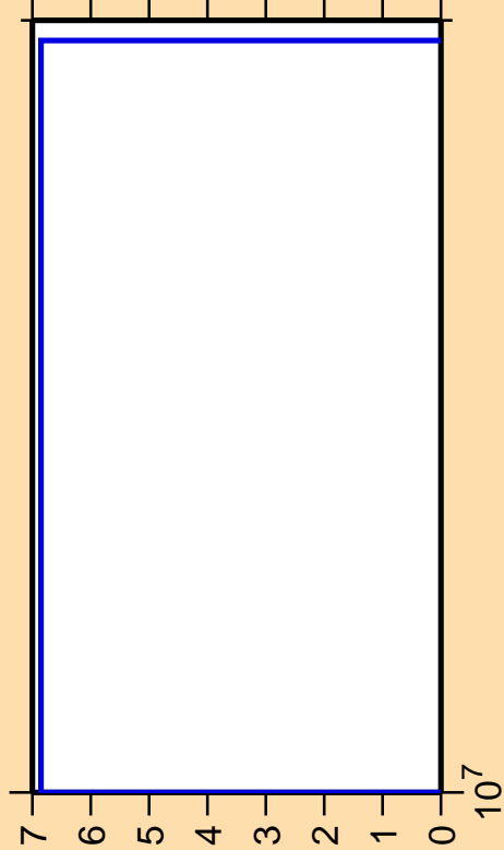
\Delta\sigma/\sigma vs. E for ^{22}\text{Mg} (mt 34)
