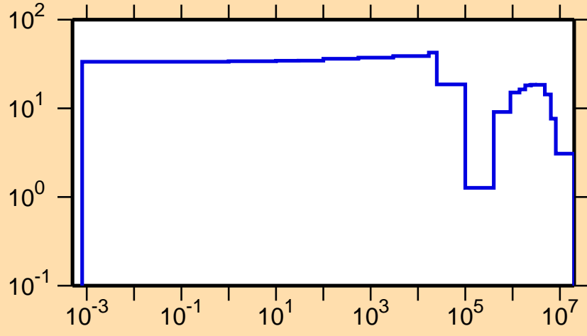
\Delta\sigma/\sigma vs. E for ^{22}\text{Mg}(n,el.)
