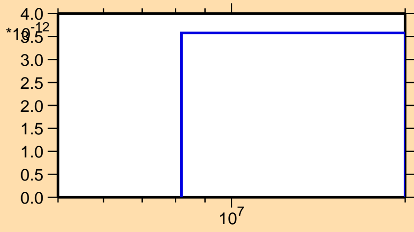
\sigma vs. E for ^{22}\text{Mg} (mt 34)
