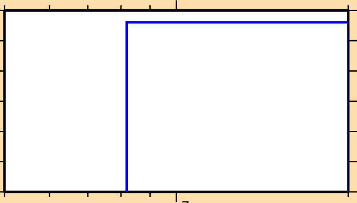
\sigma vs. E for ^{22}\text{Mg}(n,\text{pt})
