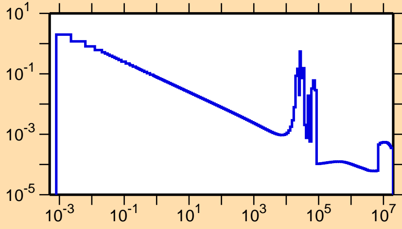
\sigma vs. E for ^{23}\text{Mg}(n,\gamma)
