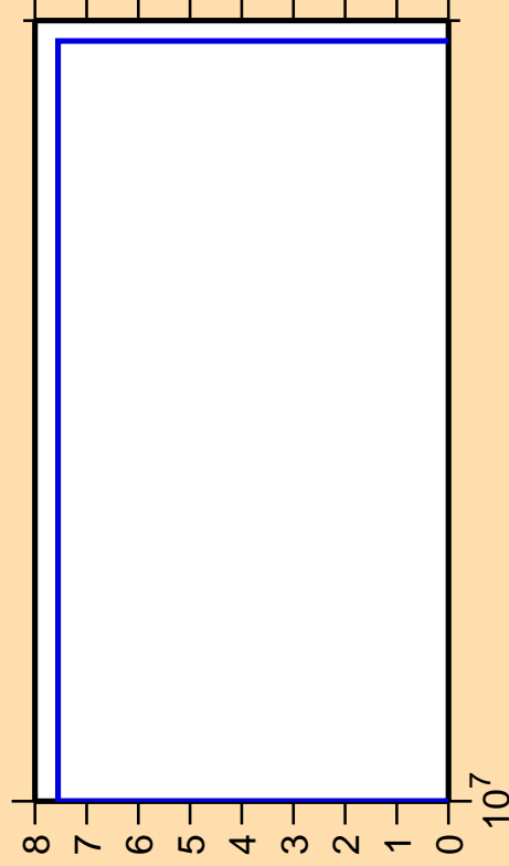
\Delta\sigma/\sigma vs. E for ^{23}\text{Mg}(n,2np)
