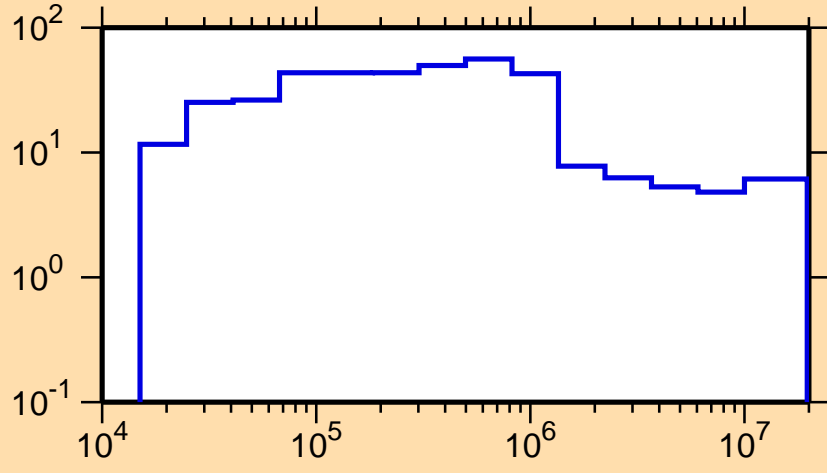
\Delta\sigma/\sigma vs. E for ^{24}\text{Mg}(n,\text{nonel.})
