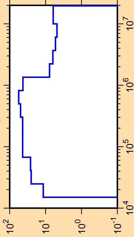
\Delta\sigma/\sigma vs. E for ^{24}\text{Mg}(n,\text{nonel.})
