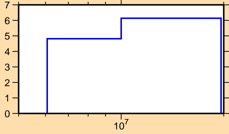
\Delta\sigma/\sigma vs. E for ^{24}\text{Mg}(n,n\text{onel.})
