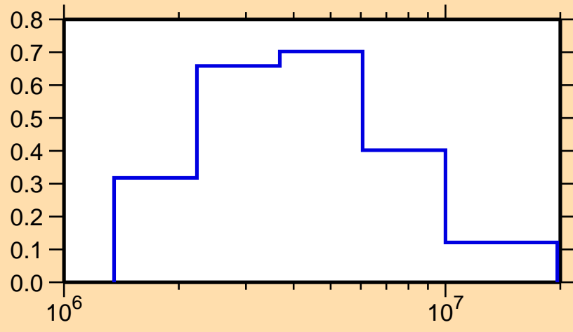
\sigma vs. E for ^{24}\text{Mg}(n,n_1)
