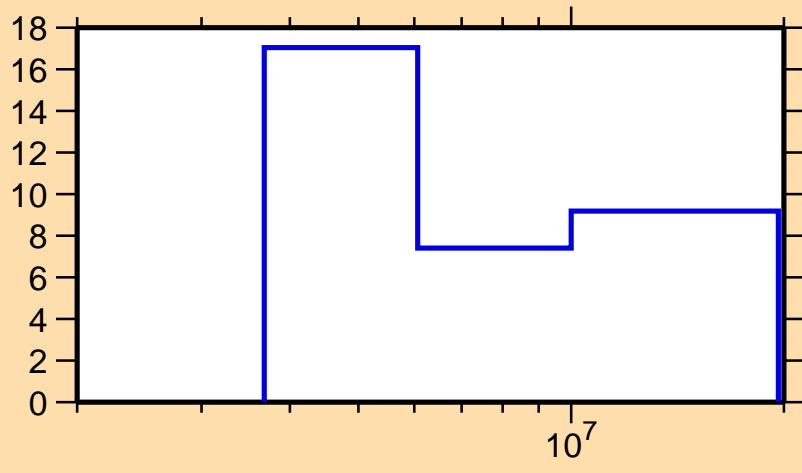
\Delta\sigma/\sigma vs. E for ^{24}\text{Mg}(n,p)
