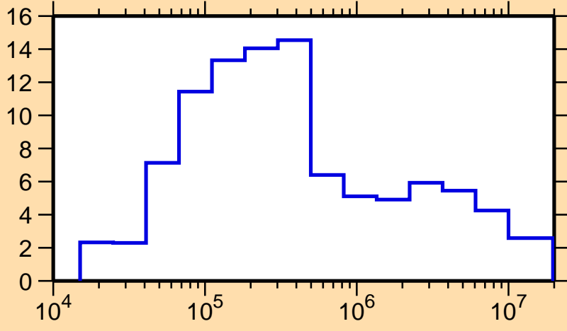
\Delta\sigma/\sigma vs. E for ^{24}\text{Mg}(n,\text{tot.})
