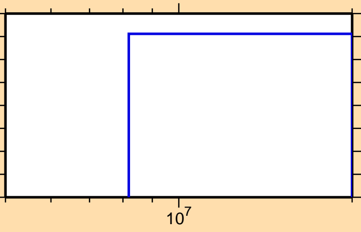
\sigma vs. E for ^{24}\text{Mg}(n,d)
