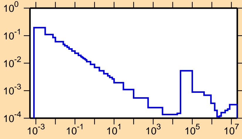
\sigma vs. E for ^{24}\text{Mg}(n,\gamma)
