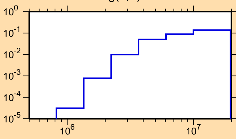
\sigma vs. E for ^{25}\text{Mg}(n,\alpha)
