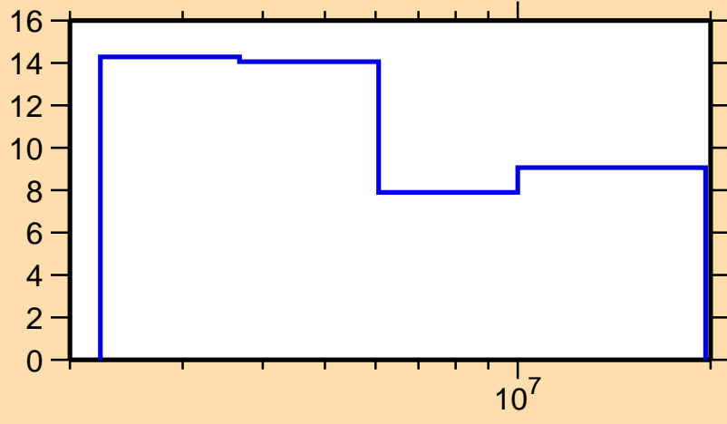
\Delta\sigma/\sigma vs. E for ^{25}\text{Mg}(n,el.)
