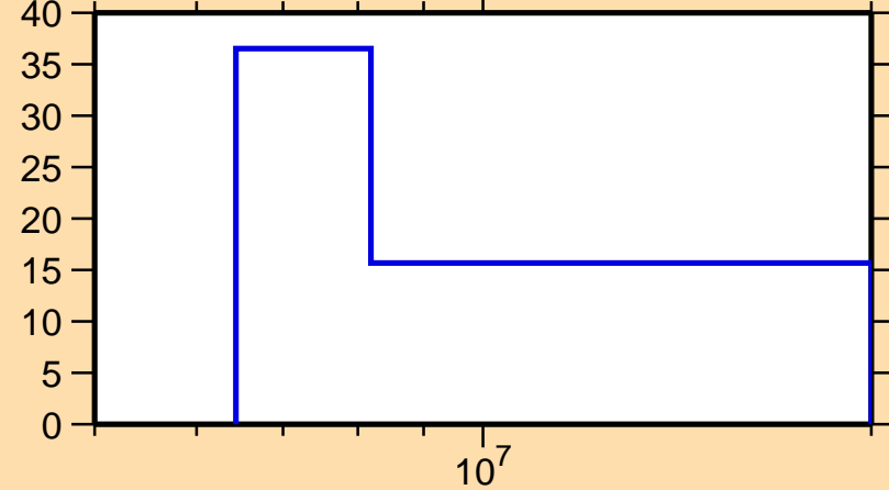
\Delta\sigma/\sigma vs. E for ^{25}\text{Mg}(n,2n)
