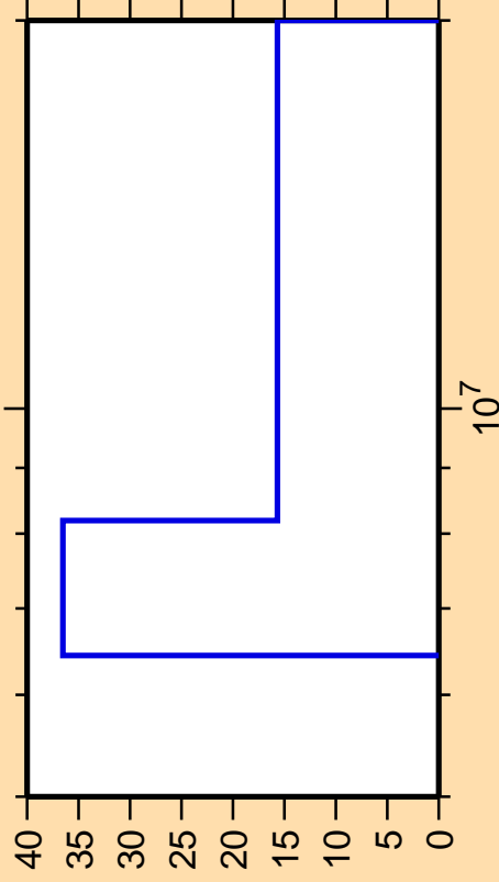
\Delta\sigma/\sigma vs. E for ^{25}\text{Mg}(n,2n)
