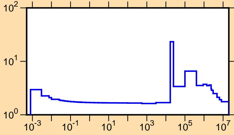
\sigma vs. E for ^{25}\text{Mg}(n,\text{tot.})
