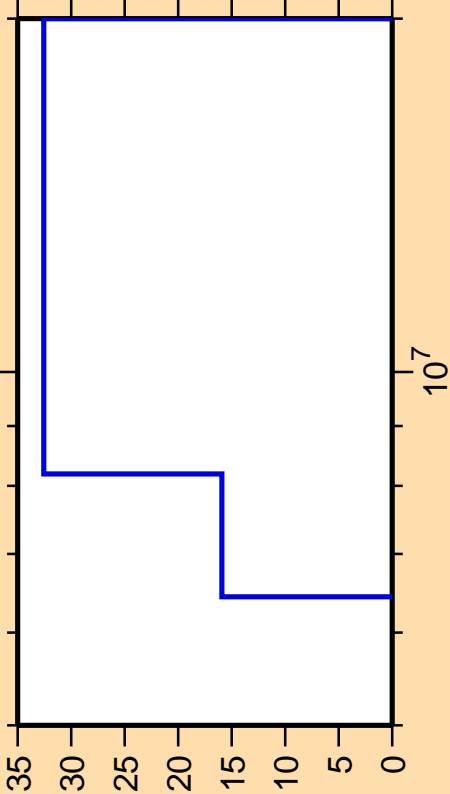
\Delta\sigma/\sigma vs. E for ^{25}\text{Mg}(n,n_1)
