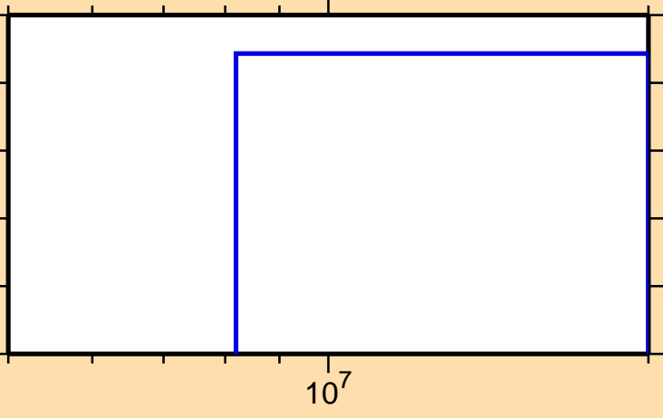
\sigma vs. E for ^{25}\text{Mg}(n,\text{He}3)
