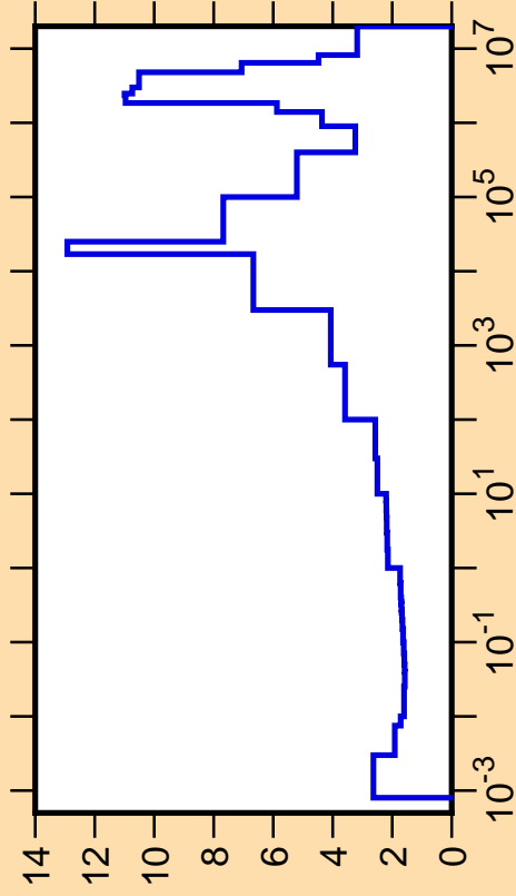
\Delta\sigma/\sigma vs. E for ^{25}\text{Mg}(n,\text{tot.})
