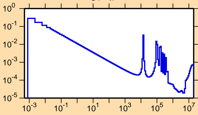
\sigma vs. E for ^{27}\text{Mg}(n,\gamma)
