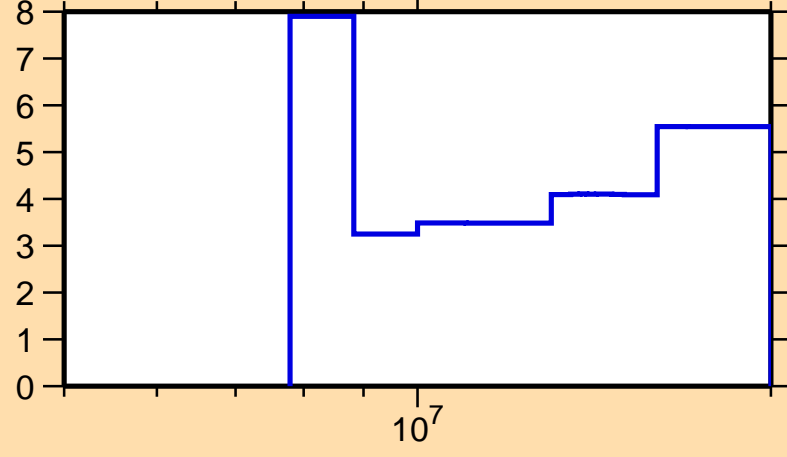
\Delta\sigma/\sigma vs. E for ^{27}\text{Mg}(n,2n)
