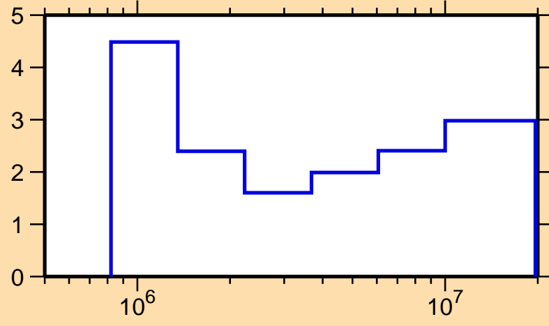
\Delta\sigma/\sigma vs. E for ^{27}\text{Mg}(n,\text{nonel.})
