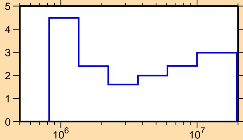
\Delta\sigma/\sigma vs. E for ^{27}\text{Mg}(n,\text{nonel.})
