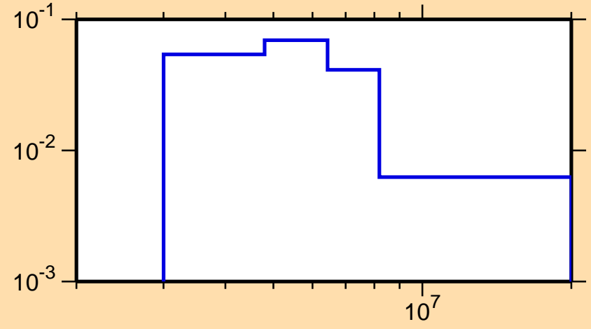
\sigma vs. E for ^{27}\text{Mg}(n,n_4)
