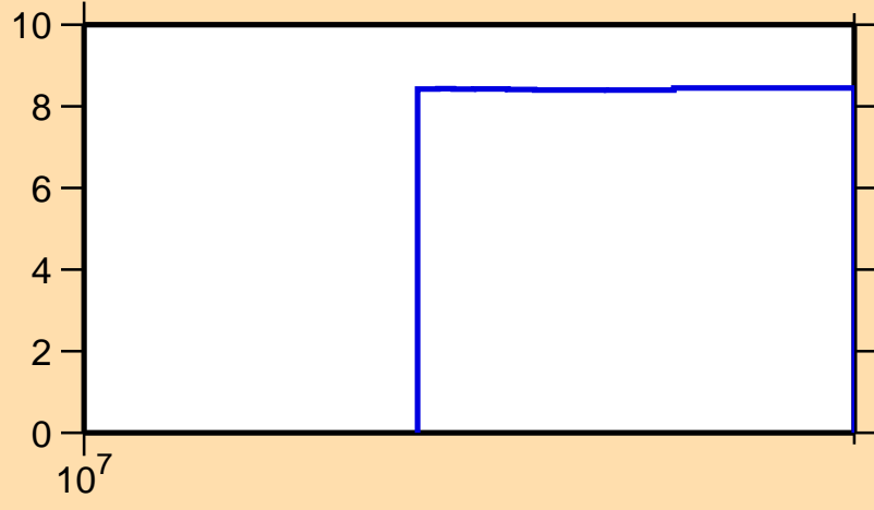
\Delta\sigma/\sigma vs. E for ^{28}\text{Mg}(n,el.)
