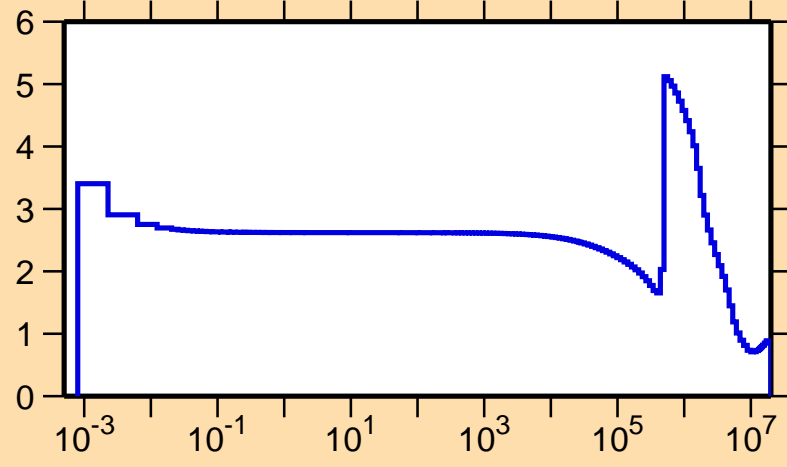
\sigma vs. E for ^{28}\text{Mg}(n,\text{el.})
