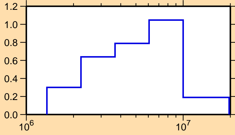
\sigma vs. E for ^{28}\text{Mg}(n,\text{inel.})
