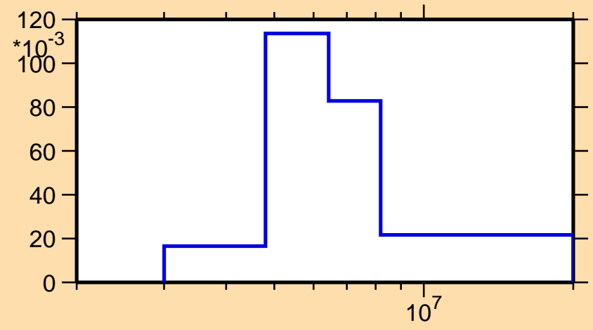
\sigma vs. E for ^{28}\text{Mg}(n,n_3)
