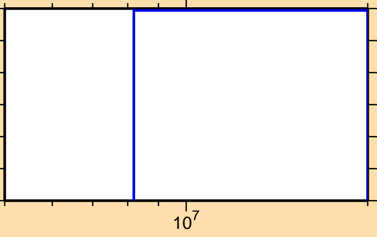
\sigma vs. E for ^{28}\text{Mg}(n,p)
