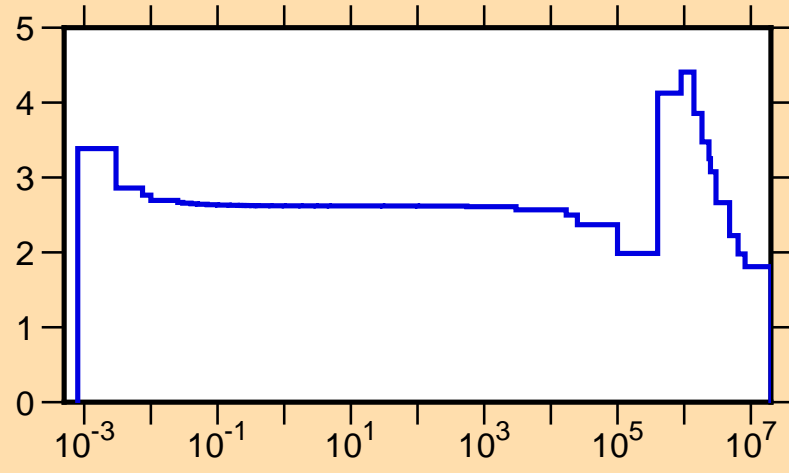
\sigma vs. E for ^{28}\text{Mg}(n,\text{tot.})
