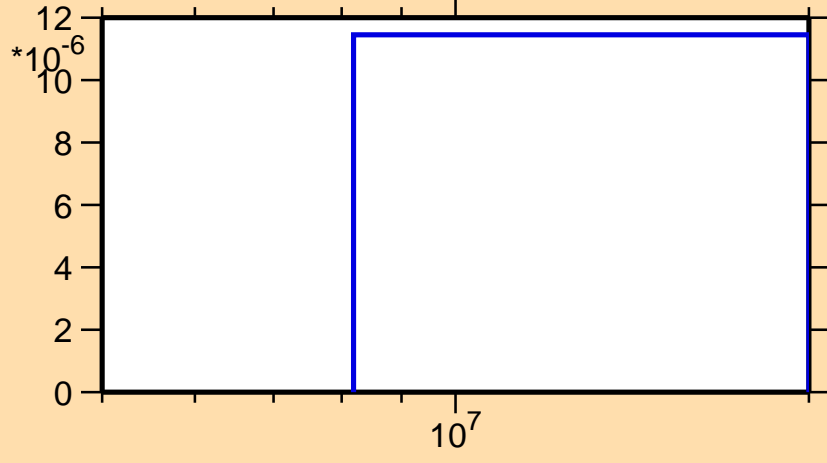
\sigma vs. E for ^{28}\text{Mg}(n,d)
