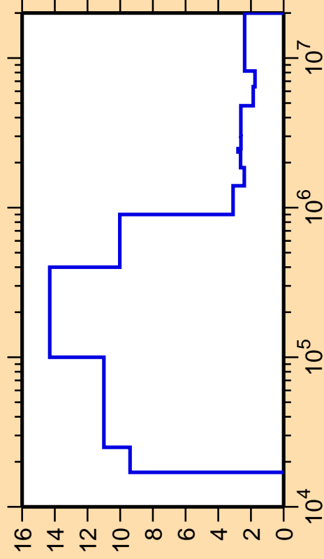
\Delta\sigma/\sigma vs. E for ^{29}\text{Mg}(n,\text{nonel.})
