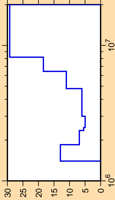
\Delta\sigma/\sigma vs. E for ^{29}\text{Mg}(n,n_4)
