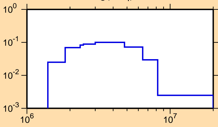
\sigma vs. E for ^{29}\text{Mg}(n,n_4)
