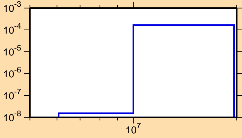
\sigma vs. E for ^{50}\text{Mn}(n,t)
