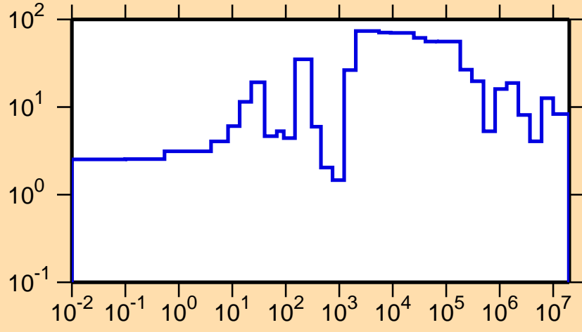
\Delta\sigma/\sigma vs. E for ^{50}\text{Mn}(n,el.)
