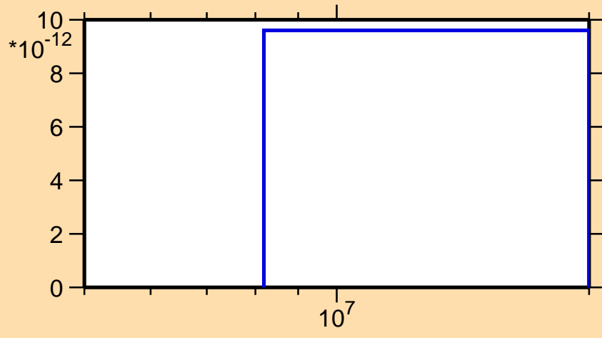
\sigma vs. E for ^{50}\text{Mn} (mt 34)
