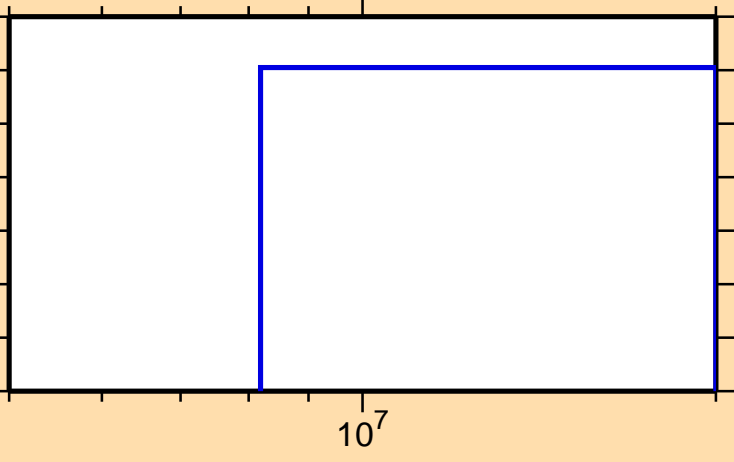
\sigma vs. E for ^{50}\text{Mn}(n,pt)
