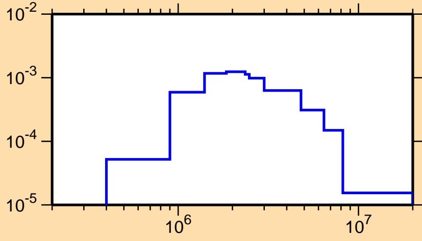
\sigma vs. E for ^{50}\text{Mn}(n,n_2)
