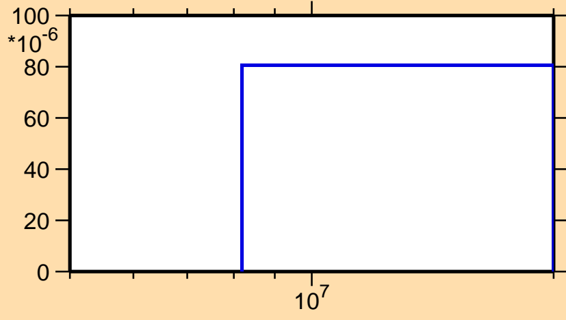
\sigma vs. E for ^{50}\text{Mn}(n,n\alpha)
