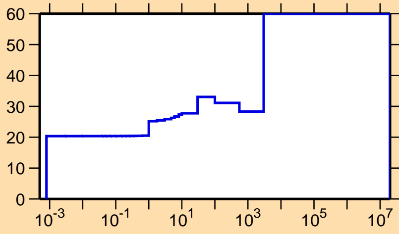
\Delta\sigma/\sigma vs. E for ^{50}\text{Mn}(n,\gamma)
