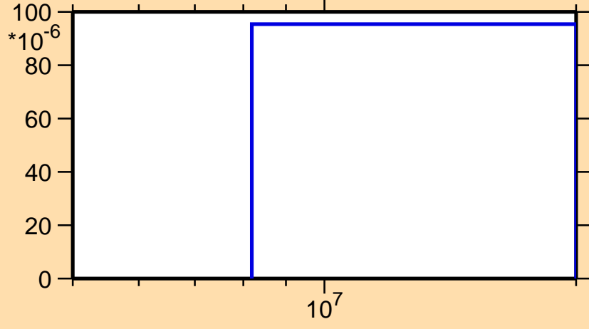
\sigma vs. E for ^{50}\text{Mn}(n,pd)
