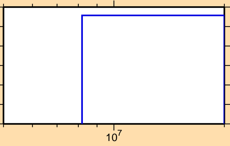
\sigma vs. E for ^{50}\text{Mn}(n,2n)
