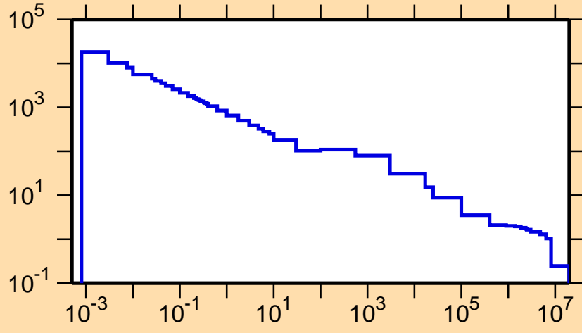
\sigma vs. E for ^{50}\text{Mn}(n,p)
