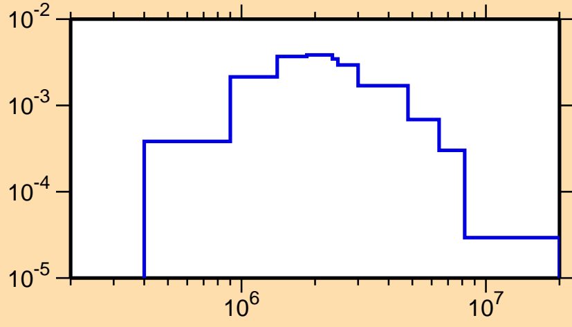
\sigma vs. E for ^{50}\text{Mn}(n,n_4)
