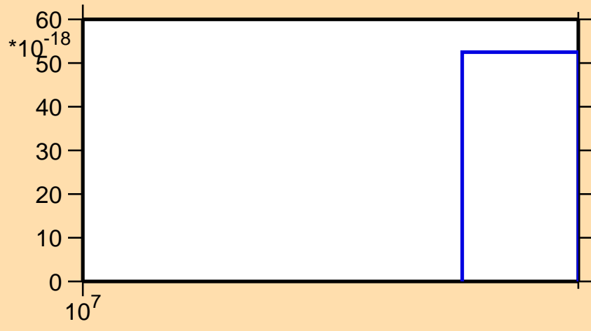
\sigma vs. E for ^{51}\text{Mn}(n,\text{pt})
