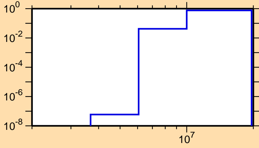
\sigma vs. E for ^{51}\text{Mn}(n,np)
