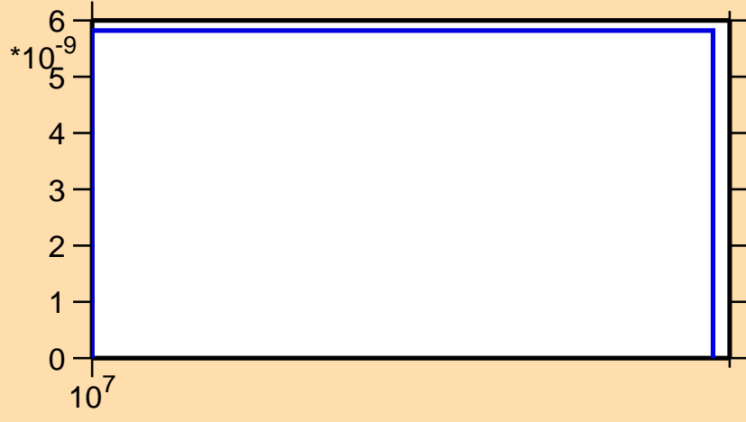
\sigma vs. E for ^{51}\text{Mn}(n,nd)
