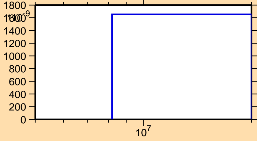
\sigma vs. E for ^{51}\text{Mn}(n,pd)
