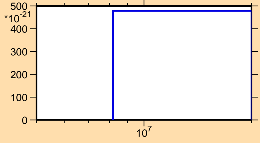
\sigma vs. E for ^{51}\text{Mn} (mt 34)
