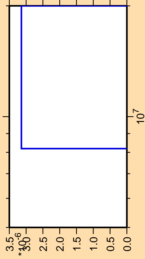
\Delta\sigma/\sigma vs. E for ^{51}\text{Mn} (mt 34)
