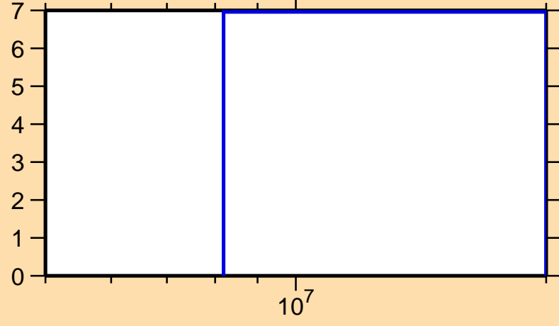
\Delta\sigma/\sigma vs. E for ^{51}\text{Mn}(n,\text{tot.})
