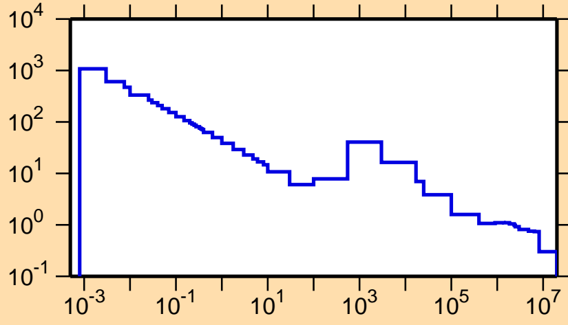
\sigma vs. E for ^{51}\text{Mn}(n,p)
