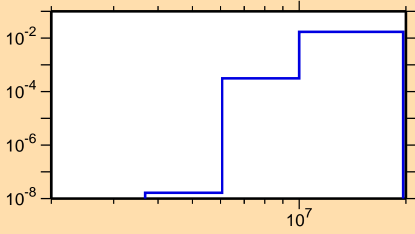
\sigma vs. E for ^{52}\text{Mn}(n,d)
