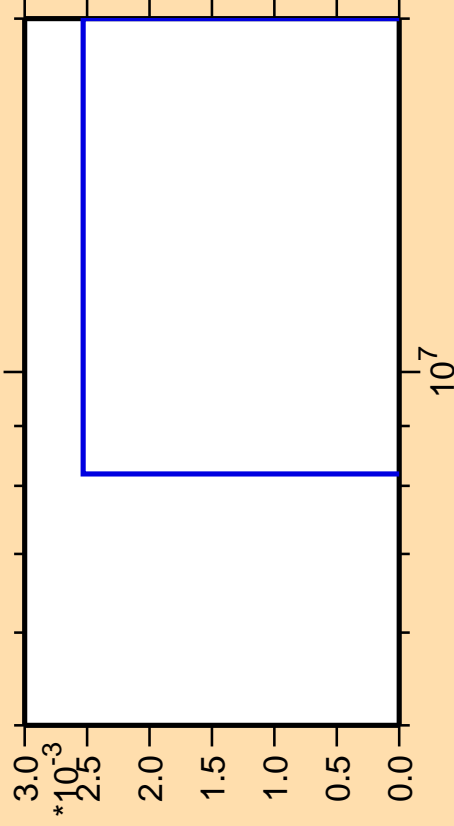
\Delta\sigma/\sigma vs. E for ^{52}\text{Mn}(\text{mt } 45)
