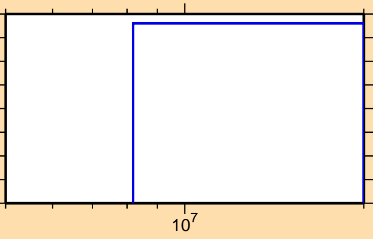
\sigma vs. E for ^{52}\text{Mn}(n,n\alpha)
