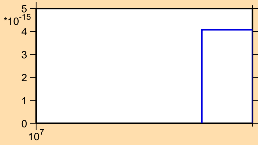
\sigma vs. E for ^{53}\text{Mn}(n,nt)
