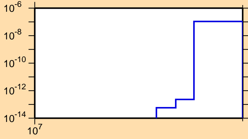
\sigma vs. E for ^{53}\text{Mn}(n,pd)
