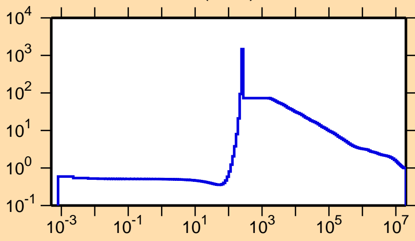
\sigma vs. E for ^{53}\text{Mn}(n,\text{el.})
