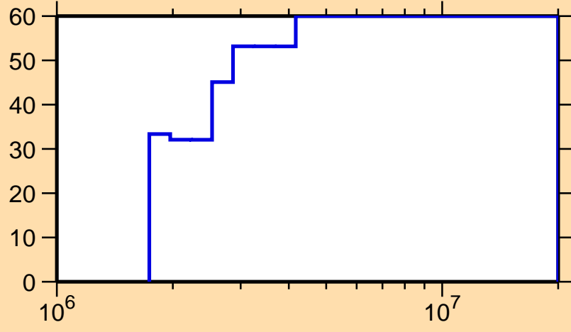
\Delta\sigma/\sigma vs. E for ^{53}\text{Mn}(n,p)
