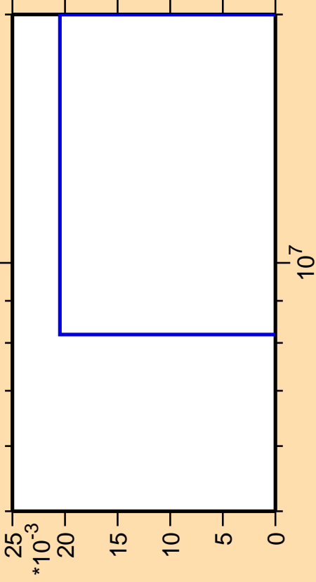
\Delta\sigma/\sigma vs. E for ^{53}\text{Mn}(\text{mt117})
