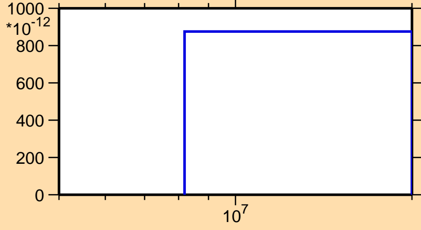
\sigma vs. E for ^{53}\text{Mn}(n,pd)
