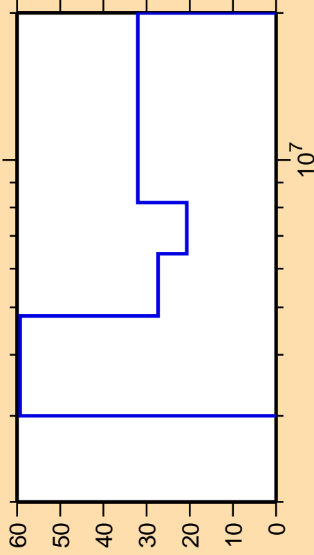
\Delta\sigma/\sigma vs. E for ^{53}\text{Mn}(n,n\text{cont.})
