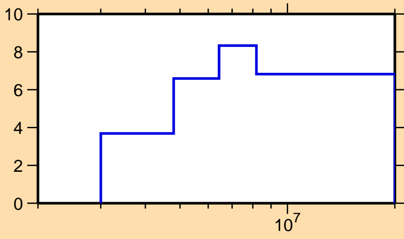
\Delta\sigma/\sigma vs. E for ^{53}\text{Mn}(n,\text{tot.})
