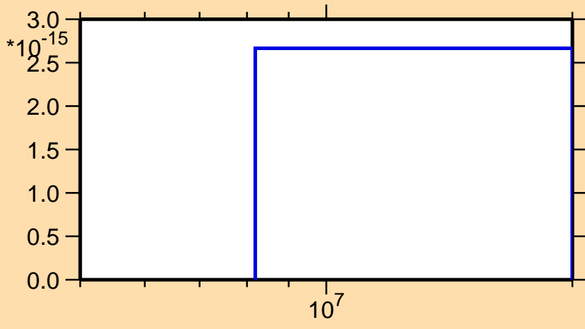
\sigma vs. E for ^{53}\text{Mn}(\text{mt117})
