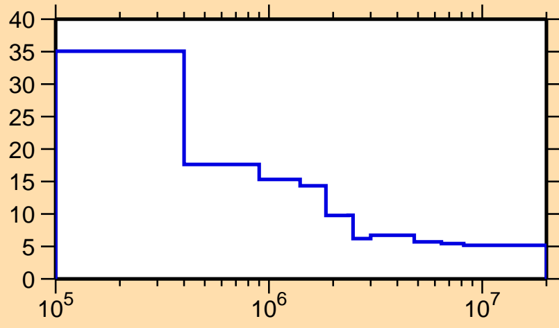
\Delta\sigma/\sigma vs. E for ^{53}\text{Mn}(n,\text{nonel.})
