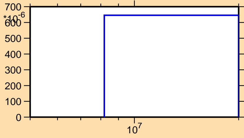
\sigma vs. E for ^{53}\text{Mn}(n,n\alpha)
