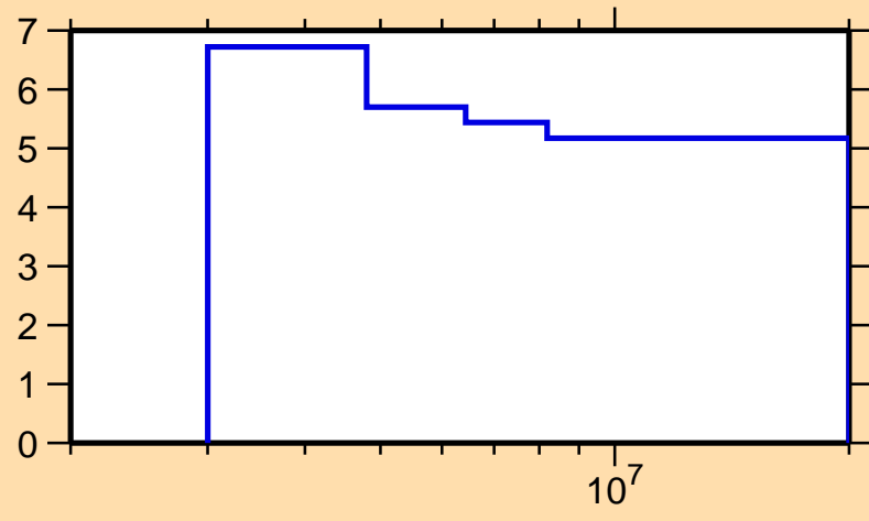
\Delta\sigma/\sigma vs. E for ^{53}\text{Mn}(n,n\text{inel.})
