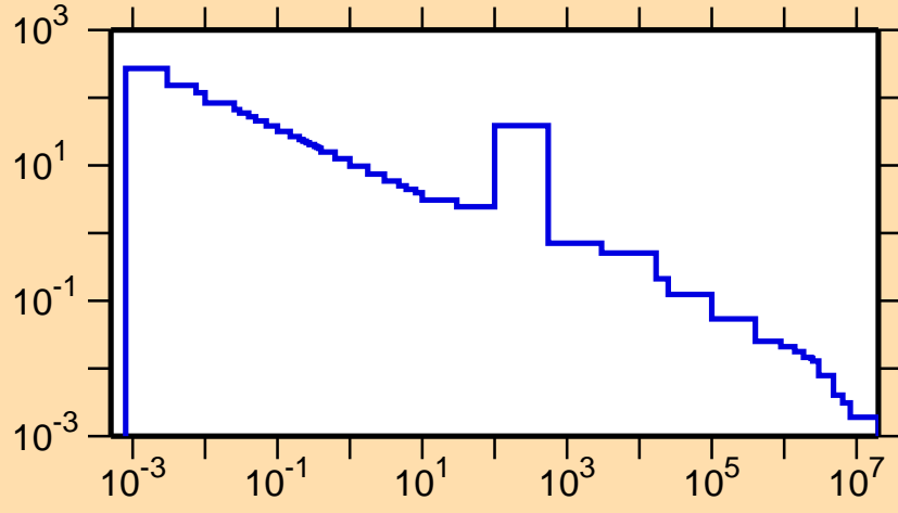
\sigma vs. E for ^{53}\text{Mn}(n,\gamma)
