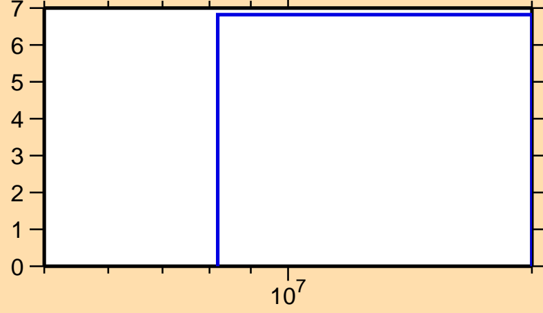
\Delta\sigma/\sigma vs. E for ^{53}\text{Mn}(n,\text{tot.})
