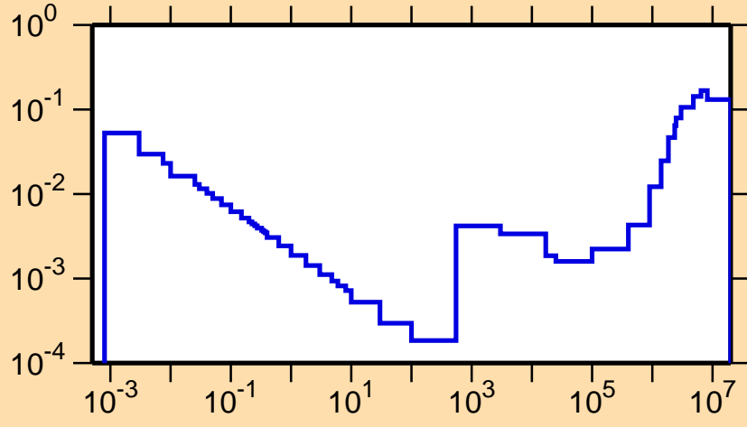
\sigma vs. E for ^{53}\text{Mn}(n,p)
