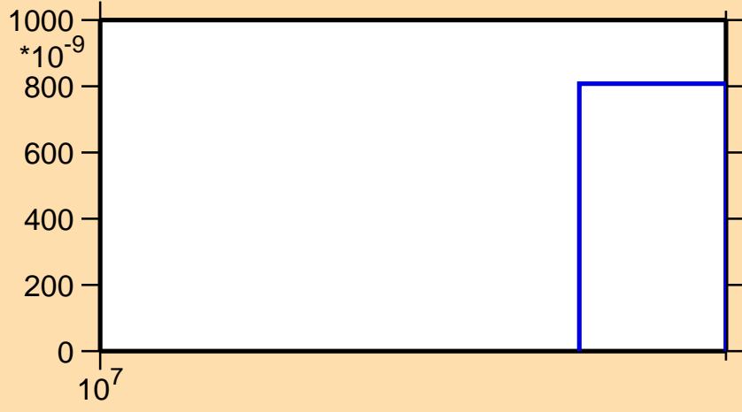
\sigma vs. E for ^{55}\text{Mn}(n,2np)
