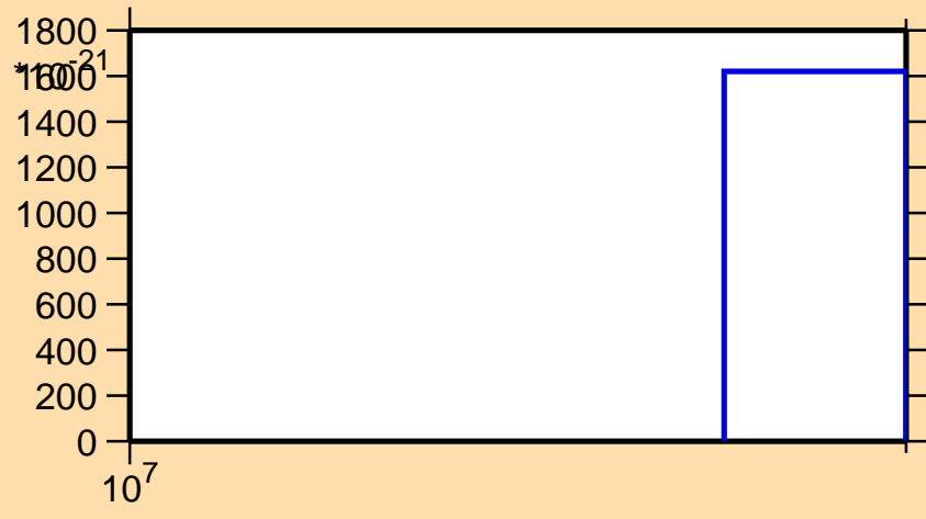
\sigma vs. E for ^{55}\text{Mn}(n,2n\alpha)
