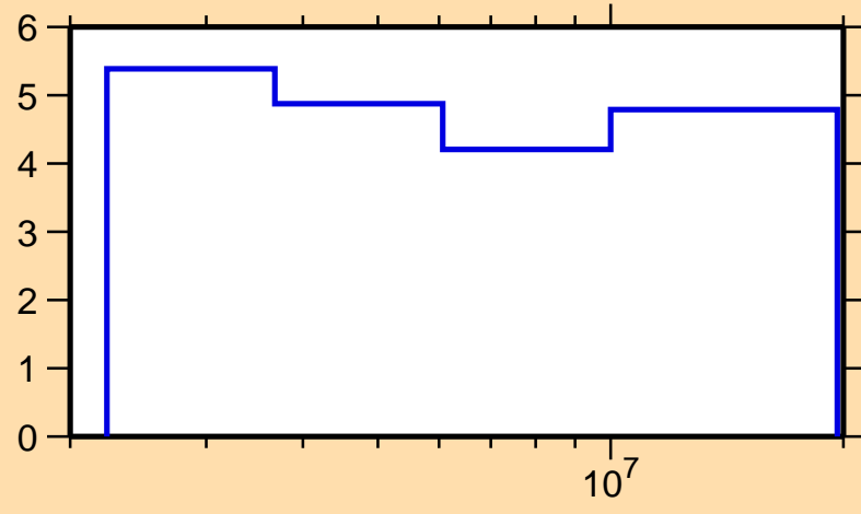
\Delta\sigma/\sigma vs. E for ^{55}\text{Mn}(n,n\text{onel.})
