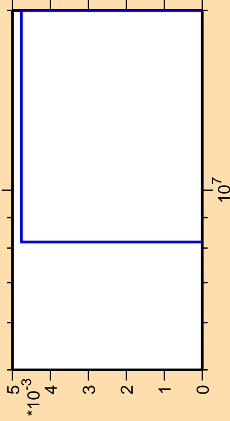
\Delta\sigma/\sigma vs. E for ^{55}\text{Mn}(\text{mt117})
