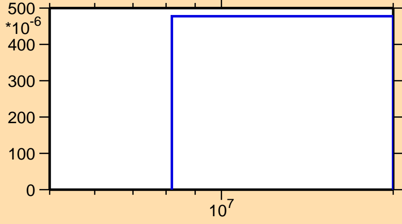
\sigma vs. E for ^{55}\text{Mn}(n,t)
