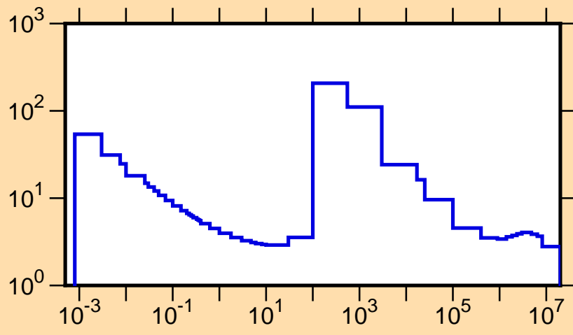
\sigma vs. E for ^{55}\text{Mn}(n,\text{tot.})
