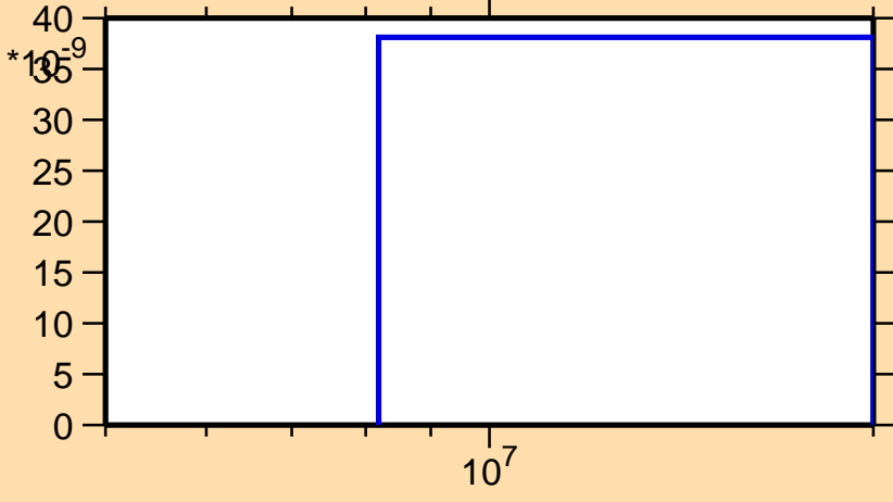
\sigma vs. E for ^{55}\text{Mn}(n,\text{nd})
