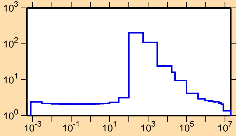
\sigma vs. E for ^{55}\text{Mn}(n,\text{el.})
