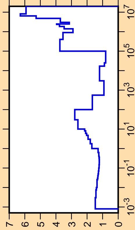
\Delta\sigma/\sigma vs. E for ^{55}\text{Mn}(n,\text{tot.})
