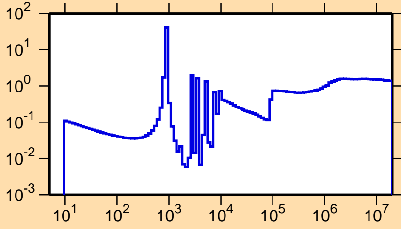
\sigma vs. E for ^{57}\text{Mn}(n,\text{nonel.})
