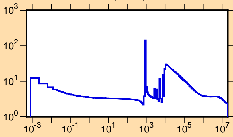
\sigma vs. E for ^{57}\text{Mn}(n,\text{tot.})
