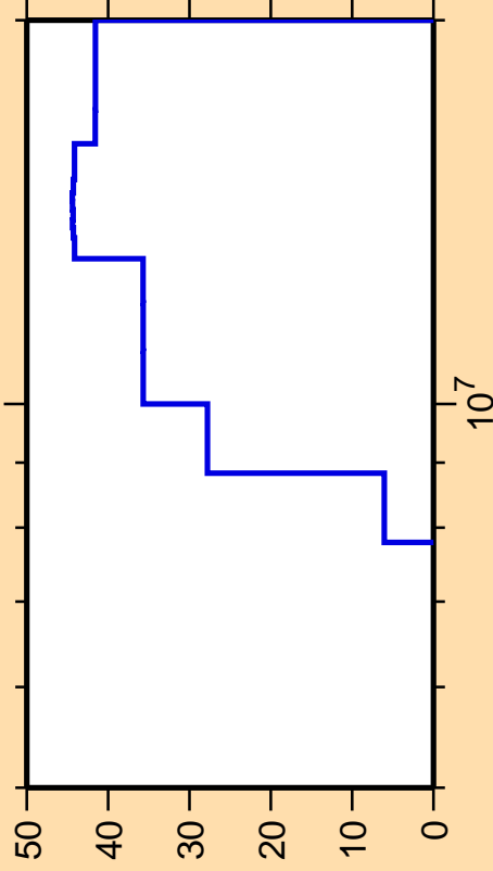
\Delta\sigma/\sigma vs. E for ^{57}\text{Mn}(n,n\text{cont.})
