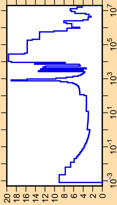
\Delta\sigma/\sigma vs. E for ^{57}\text{Mn}(n,\text{tot.})
