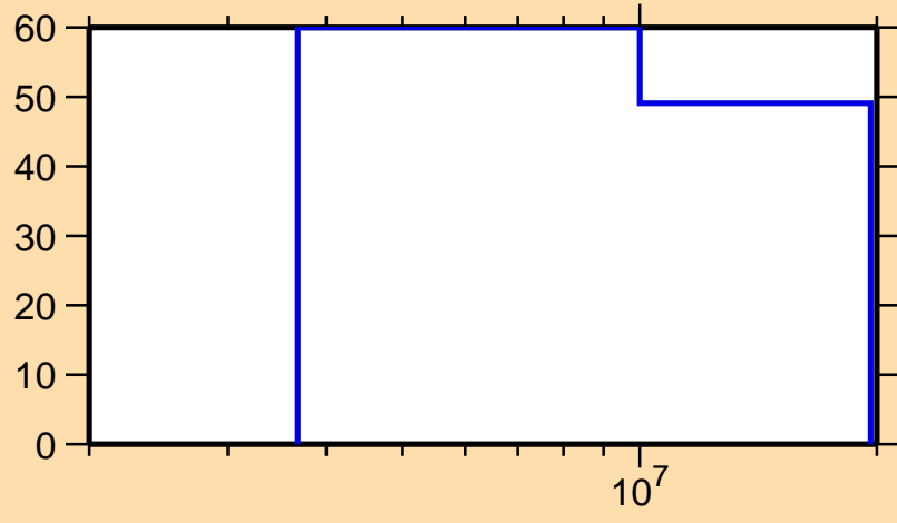
\Delta\sigma/\sigma vs. E for ^{57}\text{Mn}(n,p)
