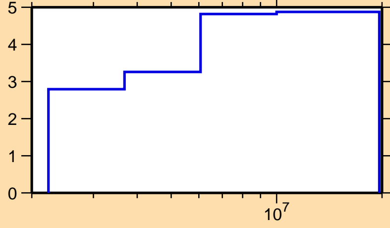
\Delta\sigma/\sigma vs. E for ^{57}\text{Mn}(n,n\text{onel.})
