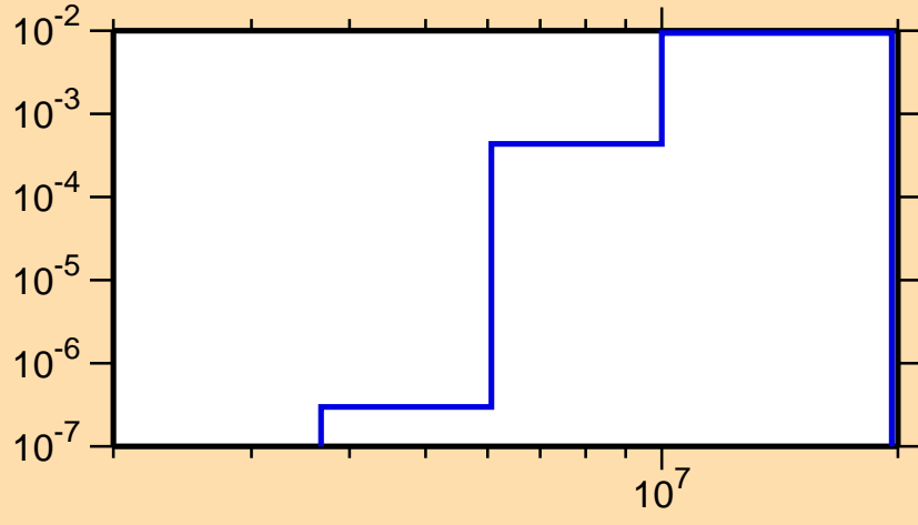
\sigma vs. E for ^{57}\text{Mn}(n,p)
