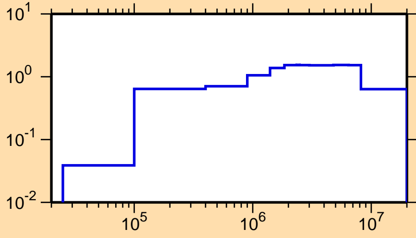
\sigma vs. E for ^{57}\text{Mn}(n,\text{inel.})
