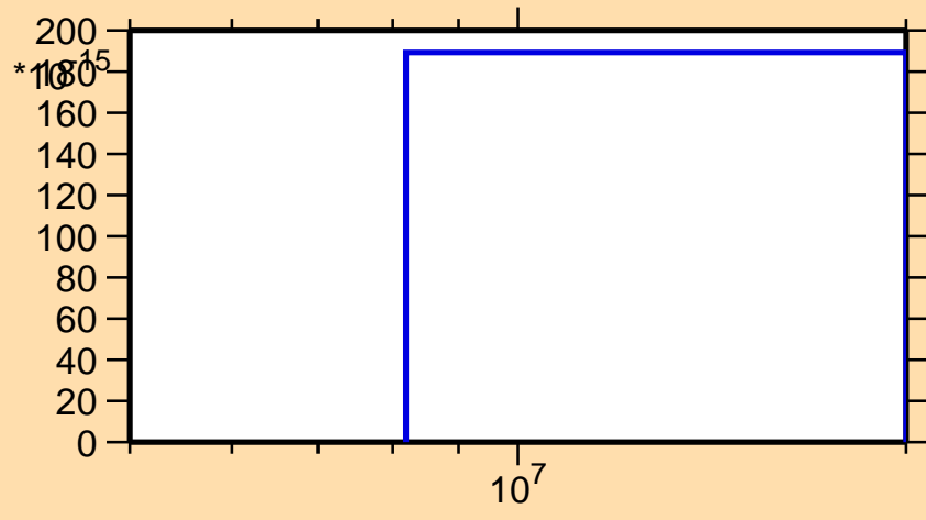
\sigma vs. E for ^{57}\text{Mn}(n,p\alpha)
