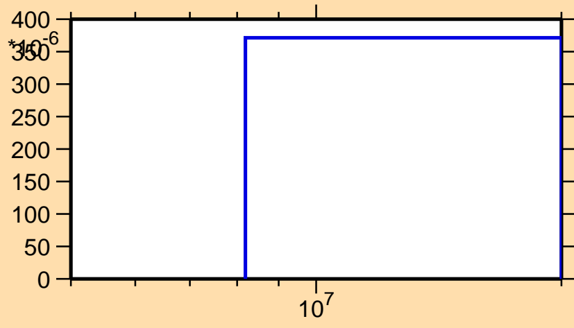
\sigma vs. E for ^{57}\text{Mn}(n,n\alpha)
