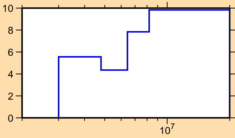
\Delta\sigma/\sigma vs. E for ^{57}\text{Mn}(n,el.)
