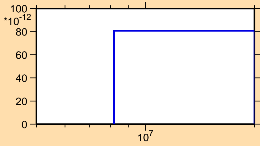
\sigma vs. E for ^{57}\text{Mn}(n,2np)
