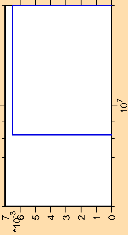
\Delta\sigma/\sigma vs. E for ^{57}\text{Mn}(n,2n\alpha)
