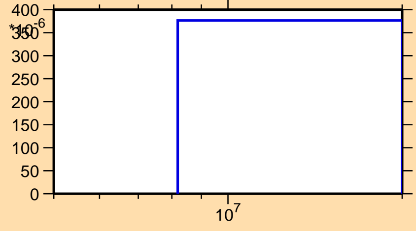
\sigma vs. E for ^{57}\text{Mn}(n,3n)
