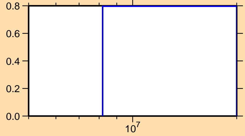
\sigma vs. E for ^{57}\text{Mn}(n,2n)
