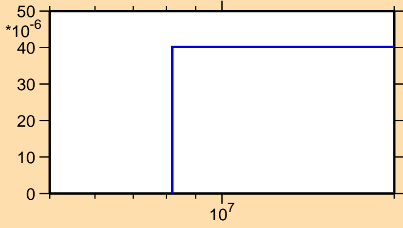
\sigma vs. E for ^{57}\text{Mn}(n,t)
