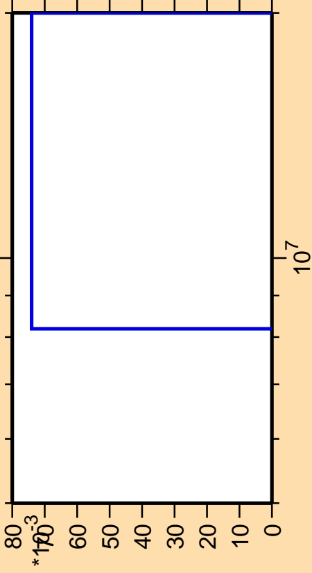
\Delta\sigma/\sigma vs. E for ^{57}\text{Mn}(n,p\alpha)
