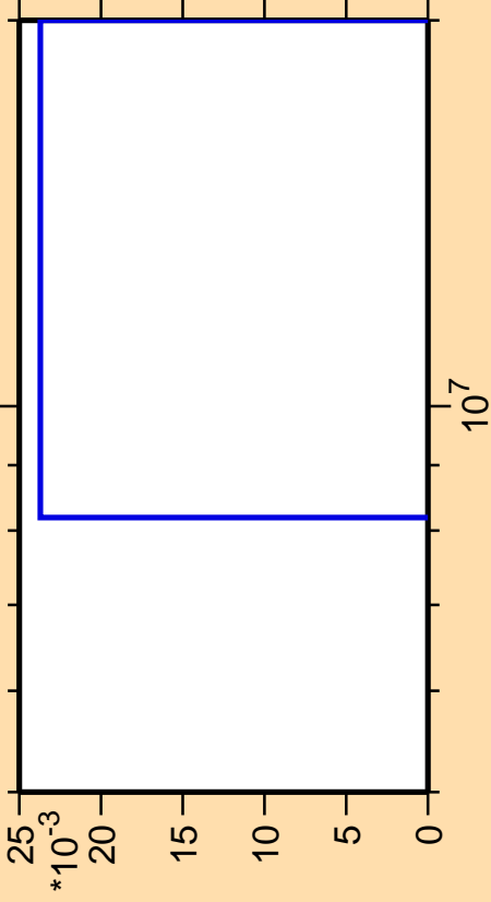
\Delta\sigma/\sigma vs. E for ^{57}\text{Mn}(n,\text{He3})
