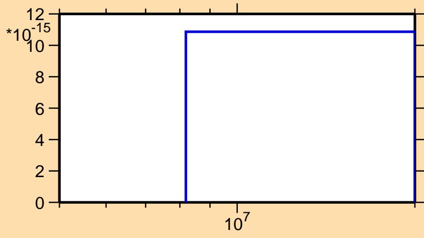
\sigma vs. E for ^{57}\text{Mn}(n,2n\alpha)
