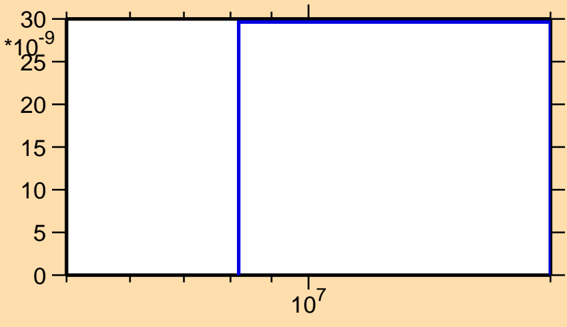
\sigma vs. E for ^{57}\text{Mn}(n,nd)
