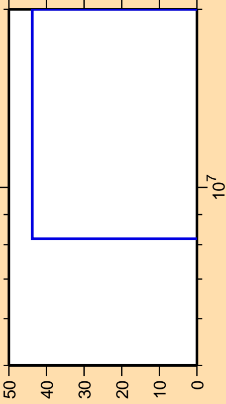
\Delta\sigma/\sigma vs. E for ^{57}\text{Mn}(n,3n)
