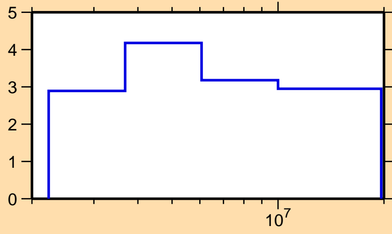
\Delta\sigma/\sigma vs. E for ^{58}\text{Mn}(n,n\text{inel.})
