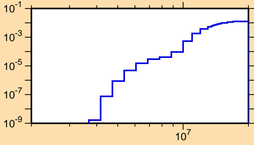
\sigma vs. E for ^{58}\text{Mn}(n,p)
