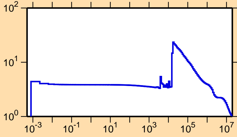
\sigma vs. E for ^{59}\text{Mn}(n,\text{el.})
