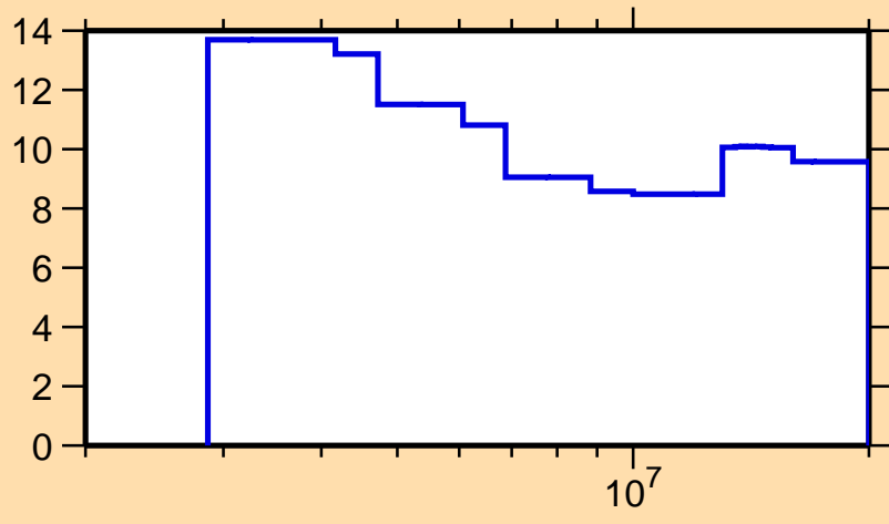
\Delta\sigma/\sigma vs. E for ^{59}\text{Mn}(n,n\text{onel.})
