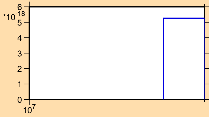
\sigma vs. E for ^{59}\text{Mn}(n,\text{He}3)
