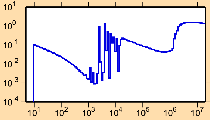
\sigma vs. E for ^{59}\text{Mn}(n,\text{nonel.})
