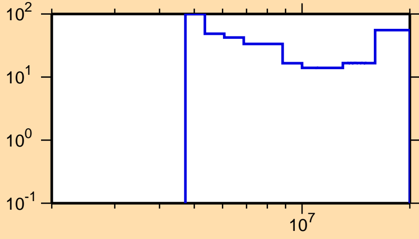
\Delta\sigma/\sigma vs. E for ^{60}\text{Mn}(n,2n)
