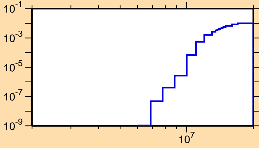
\sigma vs. E for ^{60}\text{Mn}(n,p)
