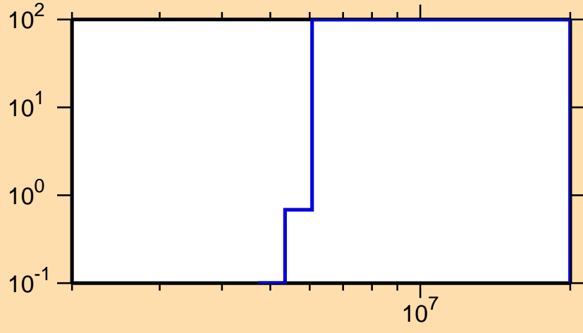
\Delta\sigma/\sigma vs. E for ^{60}\text{Mn}(n,p)
