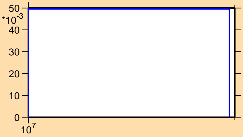
\sigma vs. E for ^{60}\text{Mn}(n,3n)
