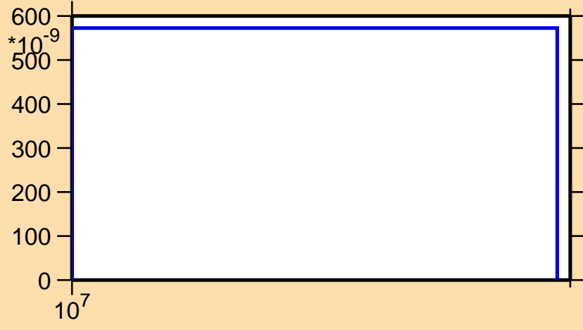
\sigma vs. E for ^{60}\text{Mn}(n,nd)
