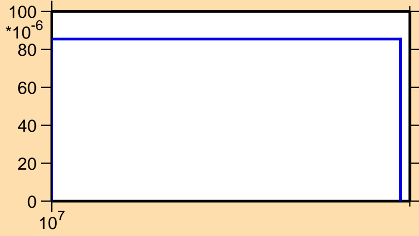
\sigma vs. E for ^{60}\text{Mn}(n,np)
