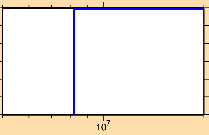
\sigma vs. E for ^{60}\text{Mn}(n,d)
