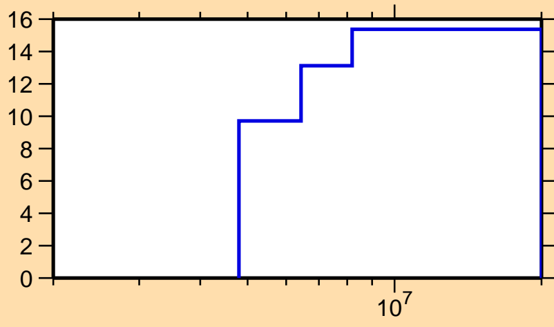
\Delta\sigma/\sigma vs. E for ^{60}\text{Mn}(n,el.)
