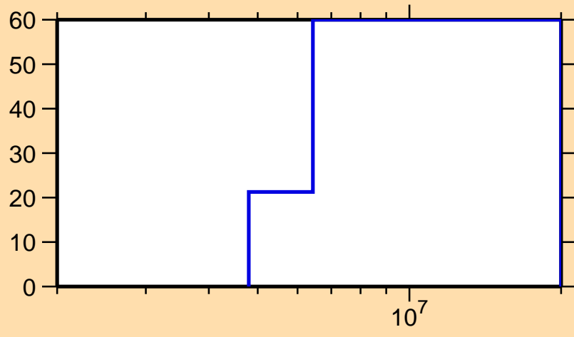
\Delta\sigma/\sigma vs. E for ^{60}\text{Mn}(n,p)
