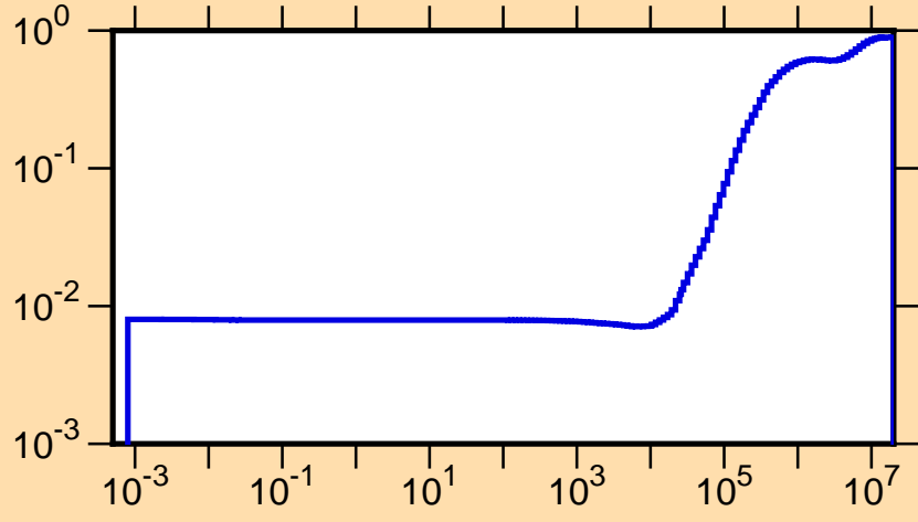
\mu vs. E for ^{84}\text{Mo}(\text{mt251})
