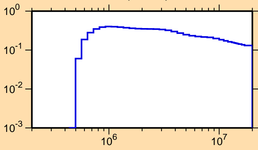
\sigma vs. E for ^{84}\text{Mo}(n,\text{inel.})
