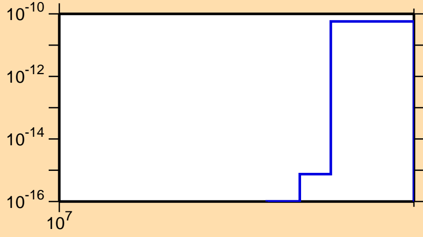
\sigma vs. E for ^{84}\text{Mo}(n,\text{nd})
