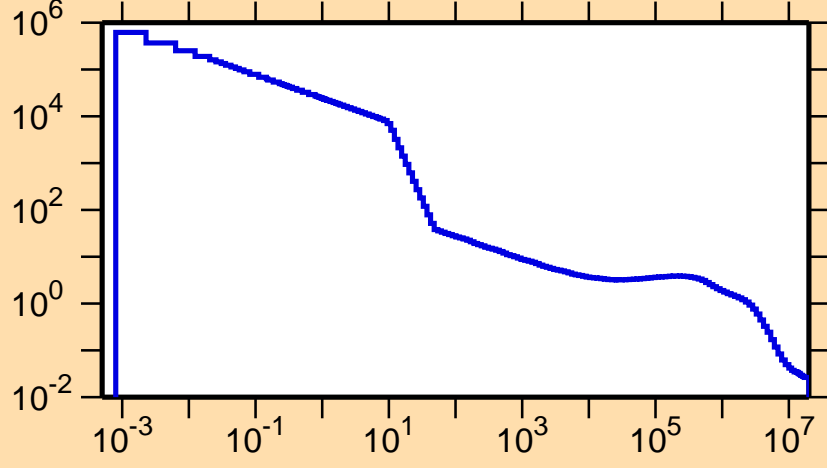
\sigma vs. E for ^{84}\text{Mo}(n,p)
