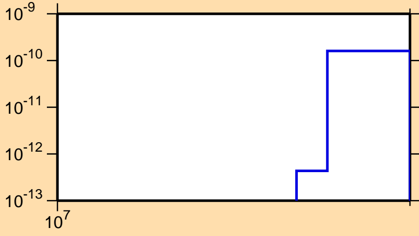
\sigma vs. E for ^{84}\text{Mo} (mt 34)
