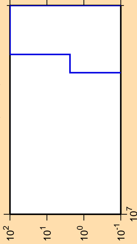
\Delta\sigma/\sigma vs. E for ^{84}\text{Mo} (mt 34)
