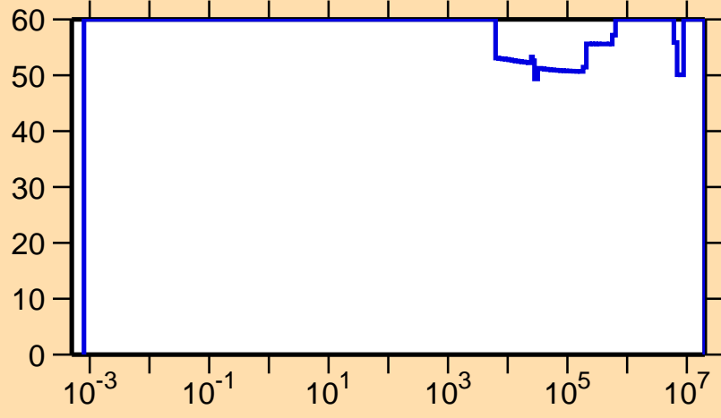
\Delta\sigma/\sigma vs. E for ^{84}\text{Mo}(n,\gamma)
