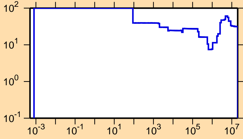
\Delta\sigma/\sigma vs. E for ^{84}\text{Mo}(n,p)
