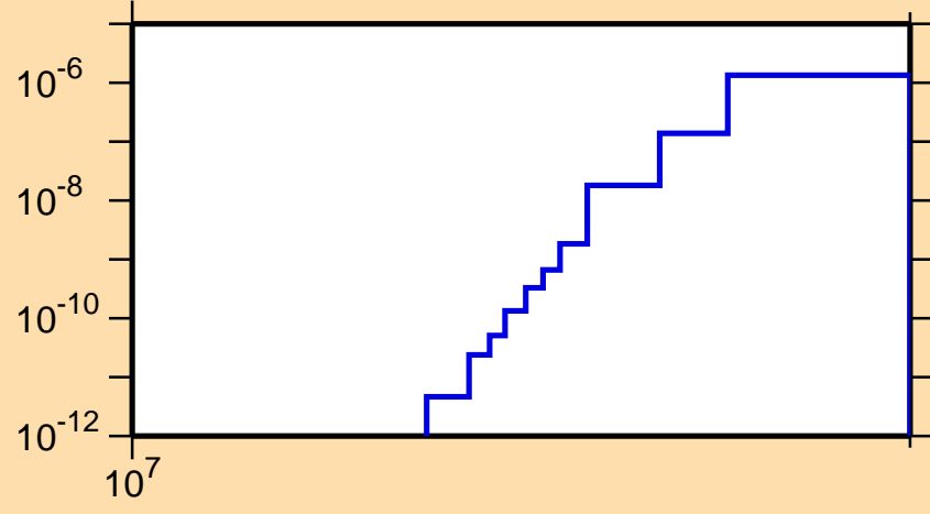
\sigma vs. E for ^{84}\text{Mo} (mt 45)
