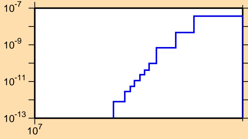
\sigma vs. E for ^{84}\text{Mo}(\text{mt117})
