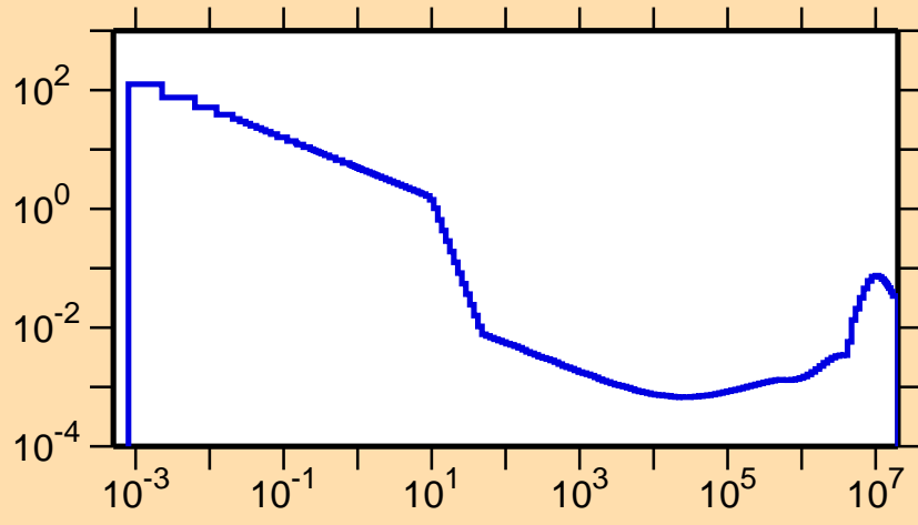
\sigma vs. E for ^{84}\text{Mo}(n,\alpha)
