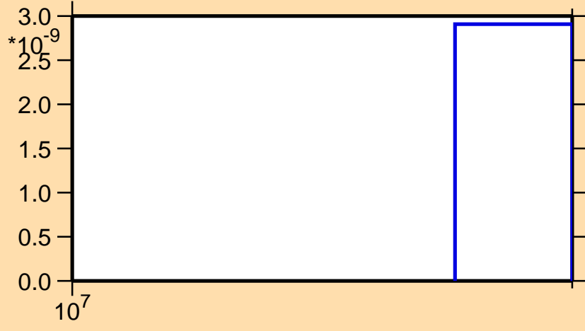
\sigma vs. E for ^{84}\text{Mo}(n,2np)
