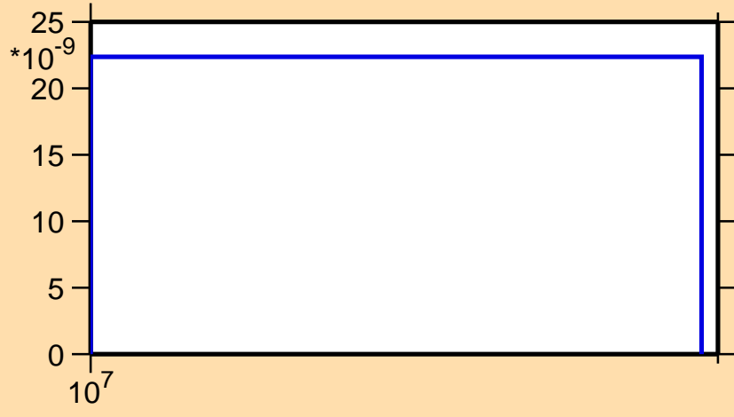
\sigma vs. E for ^{84}\text{Mo} (mt 45)
