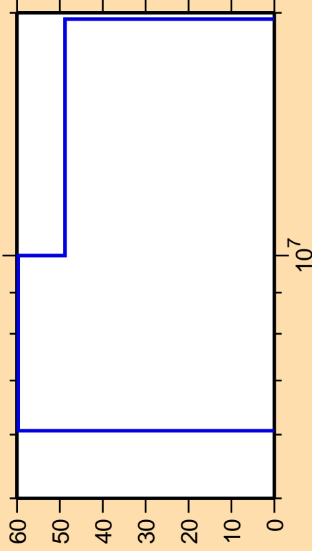
\Delta\sigma/\sigma vs. E for ^{84}\text{Mo}(n,n\alpha)
