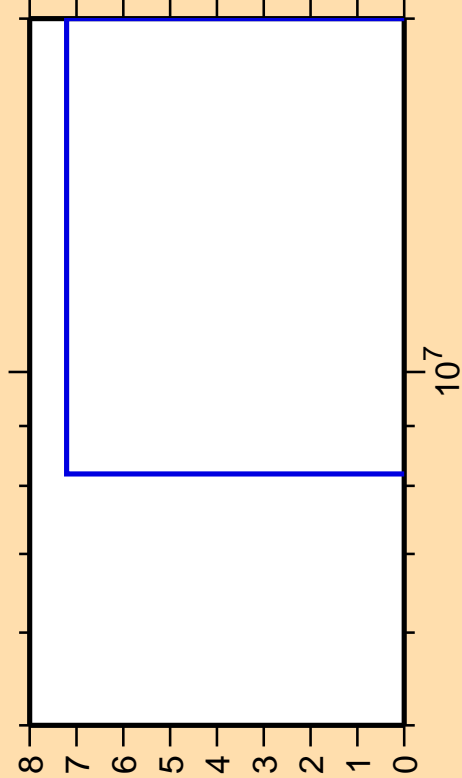
\Delta\sigma/\sigma vs. E for ^{84}\text{Mo} (mt 34)
