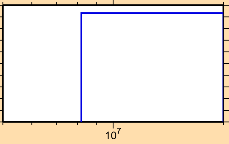
\sigma vs. E for ^{84}\text{Mo} (mt 45)
