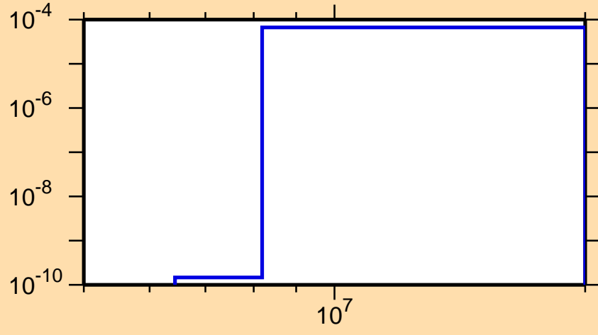
\sigma vs. E for ^{84}\text{Mo}(n,n\alpha)
