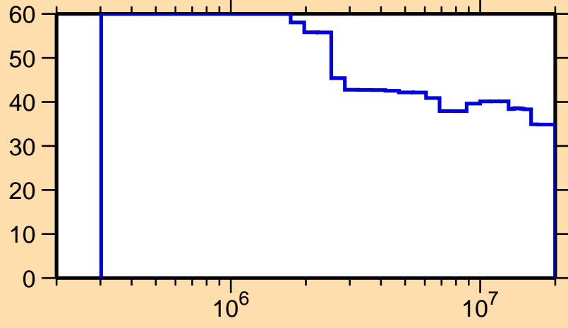
\Delta\sigma/\sigma vs. E for ^{85}\text{Mo}(n,n\text{cont.})
