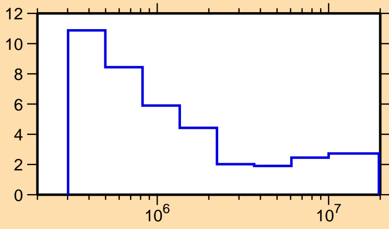
\Delta\sigma/\sigma vs. E for ^{85}\text{Mo}(n,\text{nonel.})
