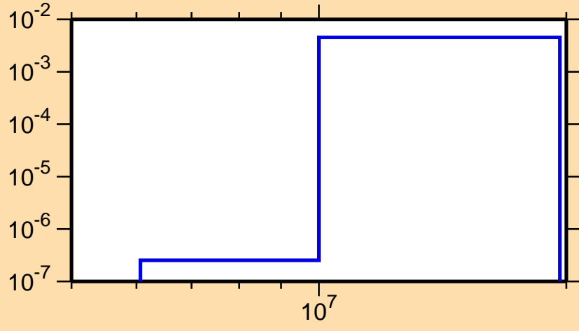
\sigma vs. E for ^{85}\text{Mo}(n,\text{pd})
