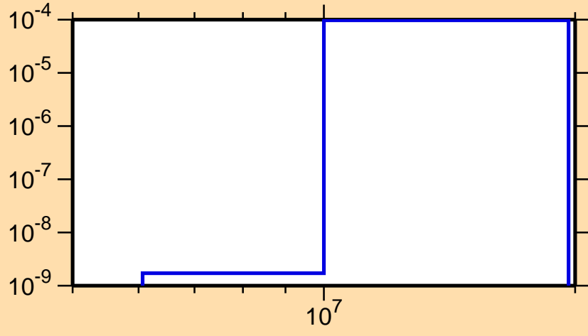
\sigma vs. E for ^{85}\text{Mo}(n,n\alpha)
