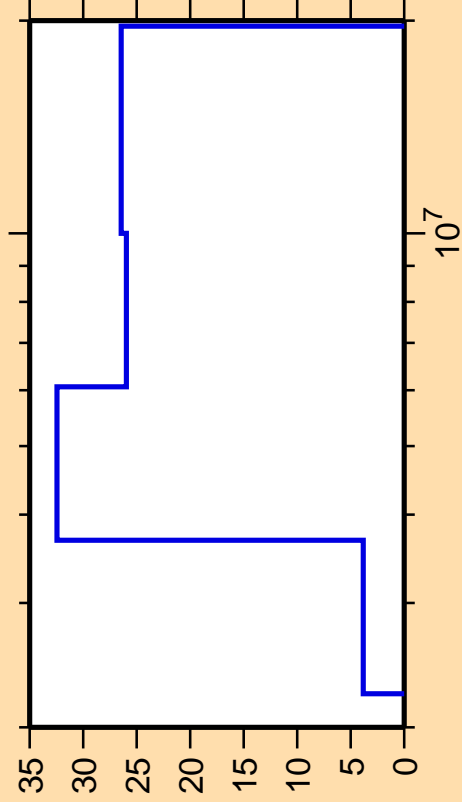
\Delta\sigma/\sigma vs. E for ^{85}\text{Mo}(n,np)
