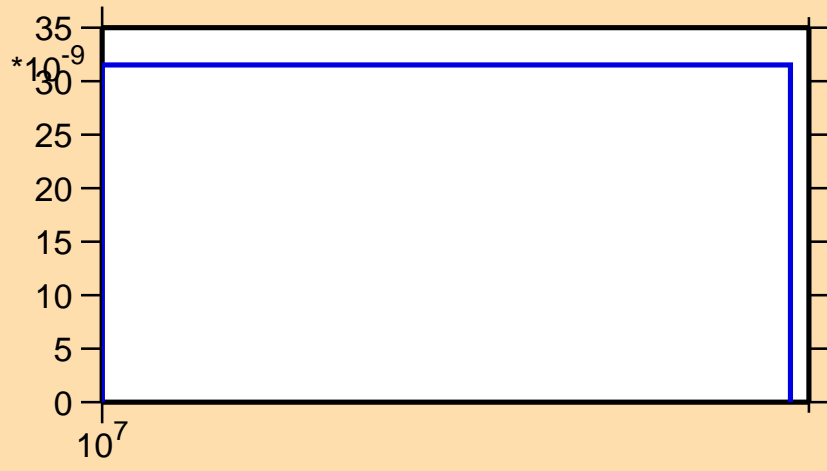
\sigma vs. E for ^{85}\text{Mo}(n,2np)
