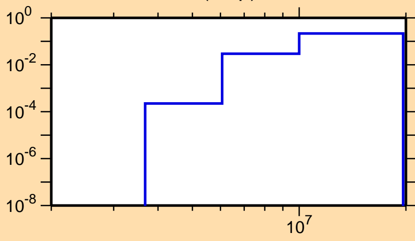
\sigma vs. E for ^{85}\text{Mo}(n,np)
