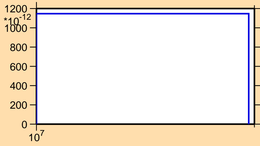
\sigma vs. E for ^{85}\text{Mo}(\text{mt117})
