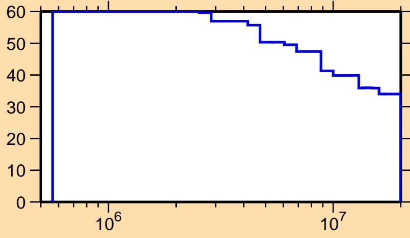
\Delta\sigma/\sigma vs. E for ^{86}\text{Mo}(n,n_1)
