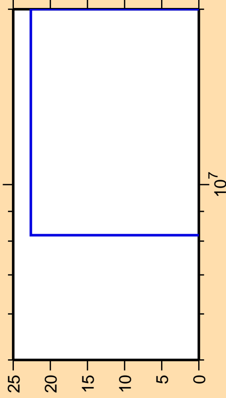
\Delta\sigma/\sigma vs. E for ^{86}\text{Mo}(n,nd)
