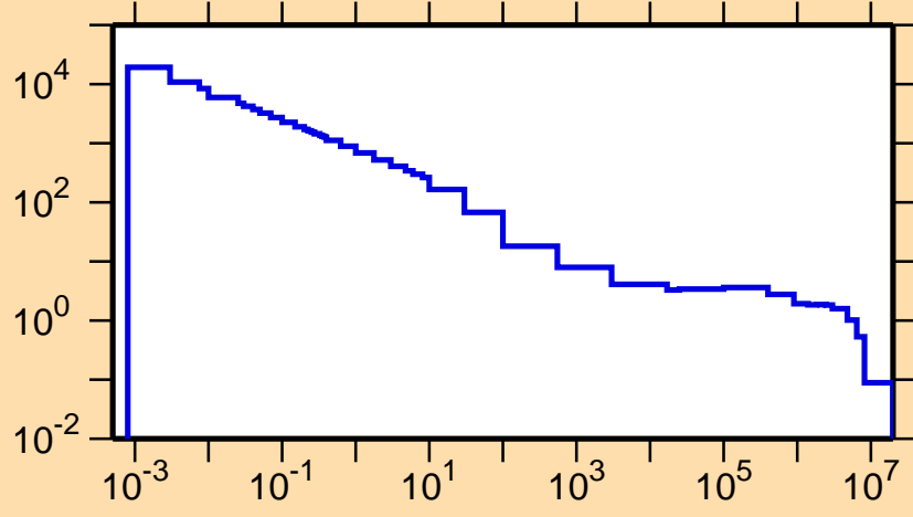
\sigma vs. E for ^{86}\text{Mo}(n,p)
