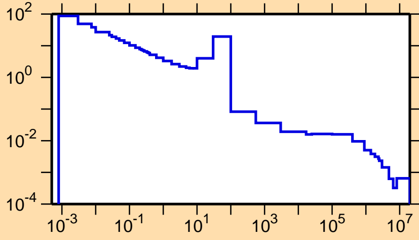
\sigma vs. E for ^{86}\text{Mo}(n,\gamma)
