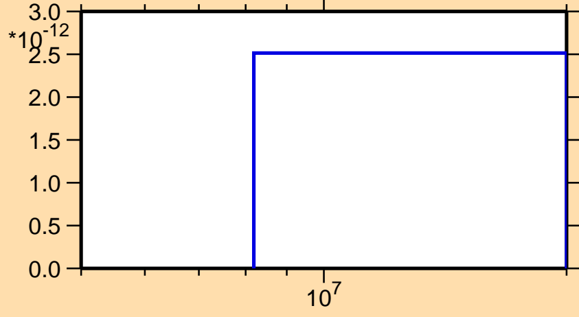
\sigma vs. E for ^{86}\text{Mo}(n,nd)
