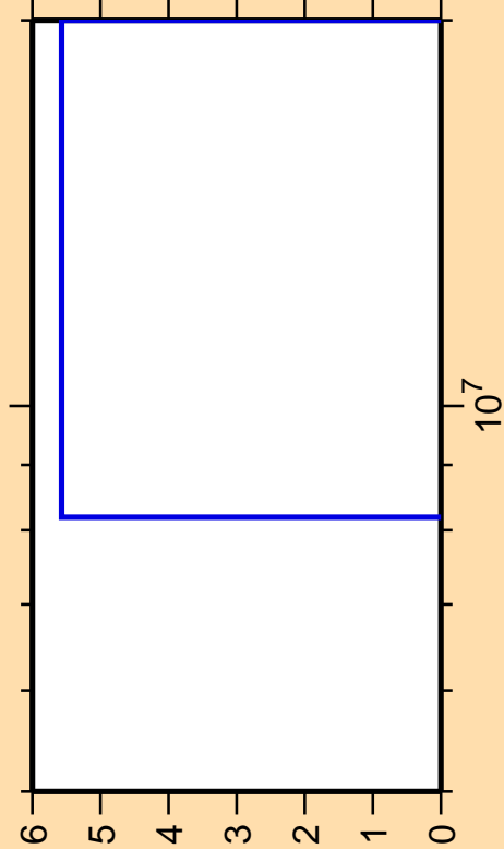
\Delta\sigma/\sigma vs. E for ^{86}\text{Mo}(n,2np)
