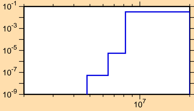
\sigma vs. E for ^{86}\text{Mo}(n,p\alpha)
