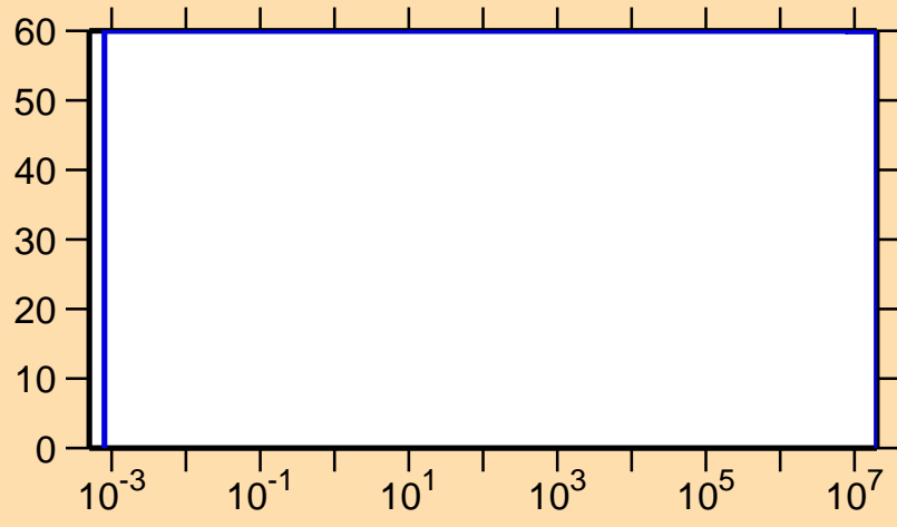
\Delta\sigma/\sigma vs. E for ^{86}\text{Mo}(n,\gamma)
