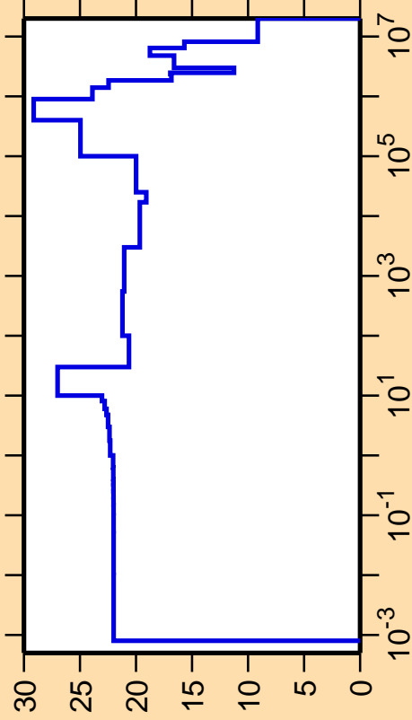
\Delta\sigma/\sigma vs. E for ^{86}\text{Mo}(n,\text{el.})
