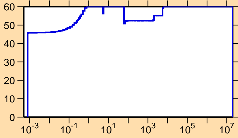
\Delta\sigma/\sigma vs. E for ^{87}\text{Mo}(n,\gamma)
