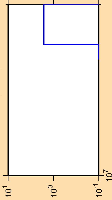
\Delta\sigma/\sigma vs. E for ^{87}\text{Mo}(n,2n\alpha)
