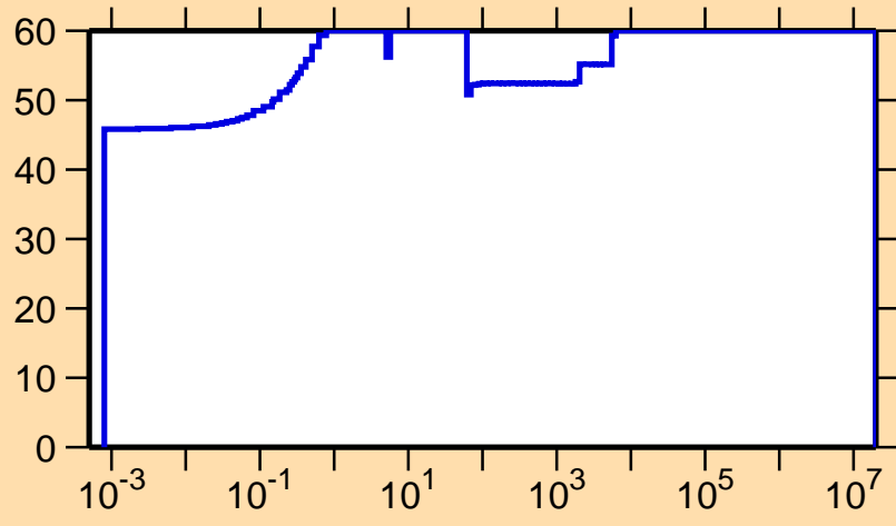
\Delta\sigma/\sigma vs. E for ^{87}\text{Mo}(n,\gamma)
