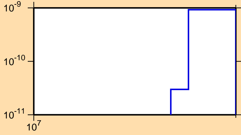
\sigma vs. E for ^{87}\text{Mo}(\text{mt117})
