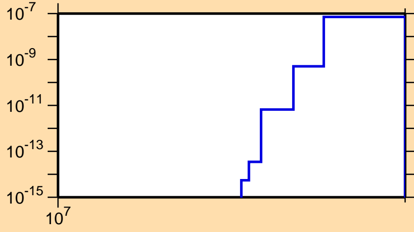
\sigma vs. E for ^{87}\text{Mo} (mt 45)
