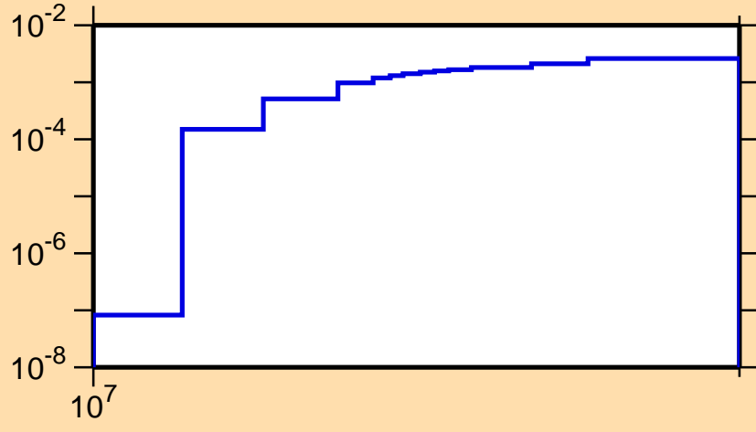
\sigma vs. E for ^{87}\text{Mo}(n,2n)
