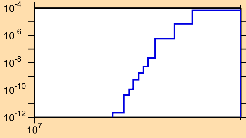
\sigma vs. E for ^{87}\text{Mo}(n,\text{pt})
