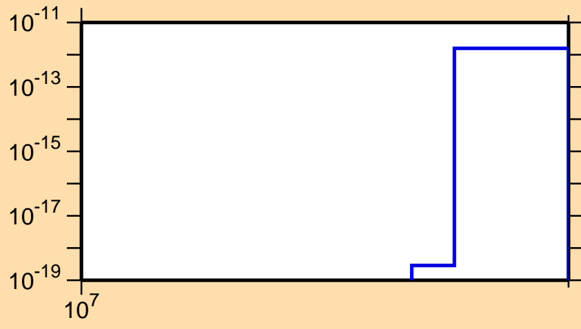
\sigma vs. E for ^{87}\text{Mo}(n,2n\alpha)
