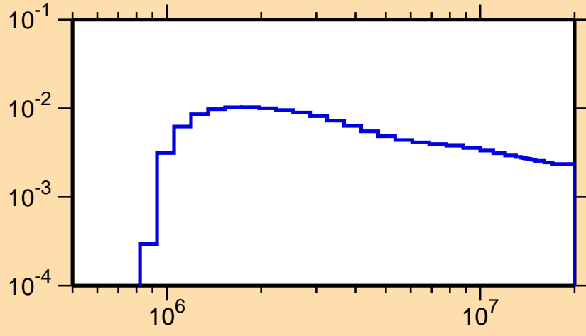
\sigma vs. E for ^{87}\text{Mo}(n,n_3)
