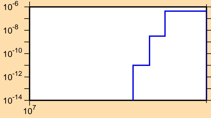
\sigma vs. E for ^{87}\text{Mo}(n,\text{nd})
