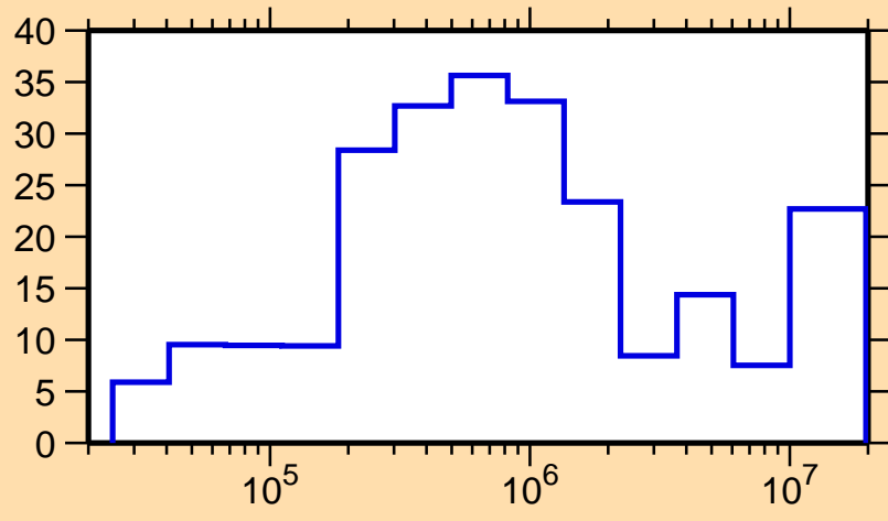
\Delta\sigma/\sigma vs. E for ^{87}\text{Mo}(n,\text{el.})
