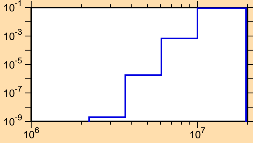
\sigma vs. E for ^{87}\text{Mo}(n,p\alpha)
