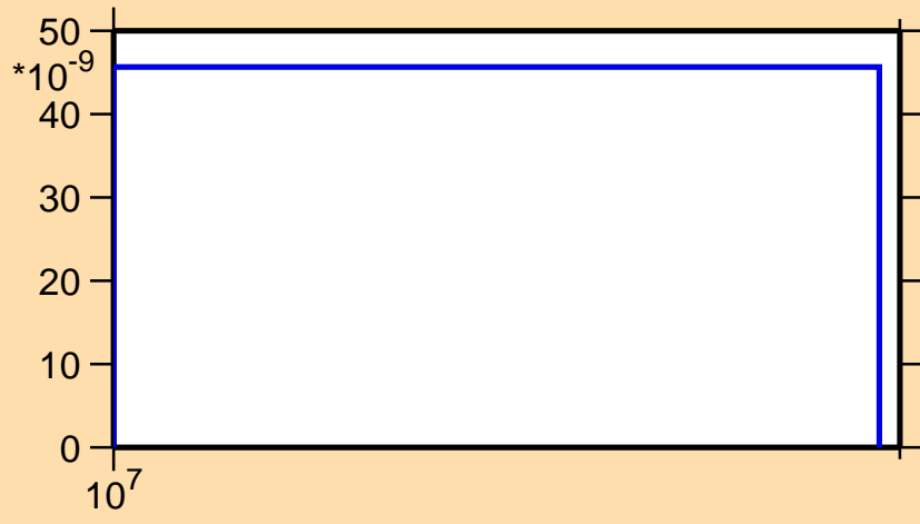
\sigma vs. E for ^{87}\text{Mo}(n,2np)
