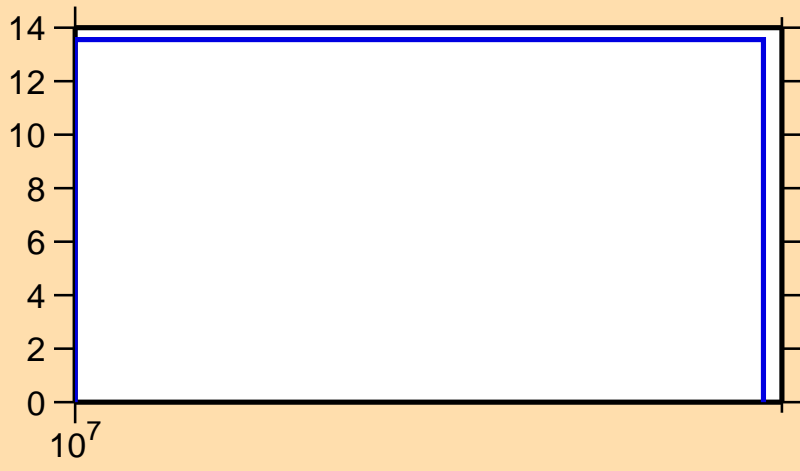
\Delta\sigma/\sigma vs. E for ^{87}\text{Mo}(n,\text{tot.})
