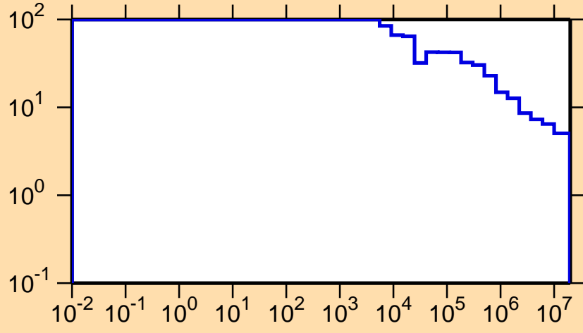
\Delta\sigma/\sigma vs. E for ^{87}\text{Mo}(n,\text{nonel.})
