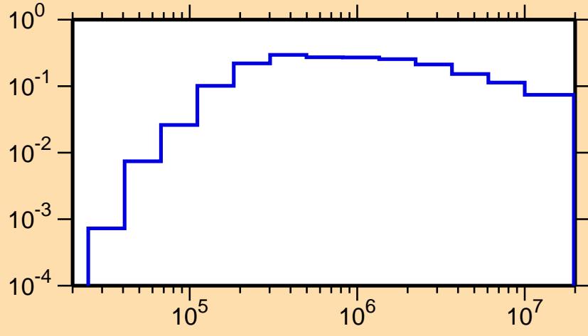
\sigma vs. E for ^{87}\text{Mo}(n,\text{inel.})
