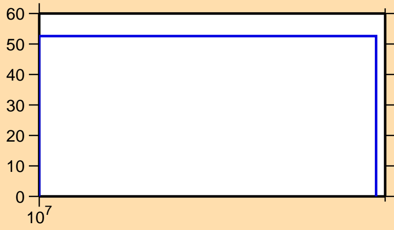
\Delta\sigma/\sigma vs. E for ^{87}\text{Mo}(n,\text{inel.})
