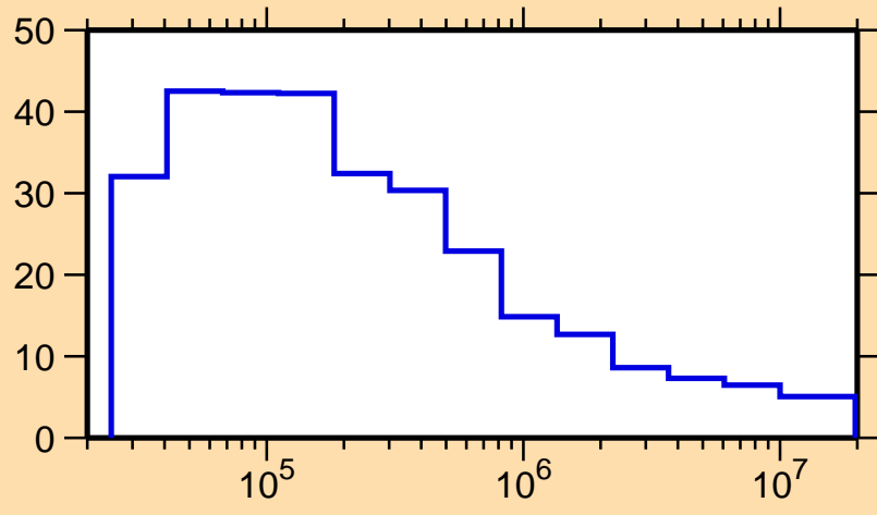
\Delta\sigma/\sigma vs. E for ^{87}\text{Mo}(n,\text{nonel.})
