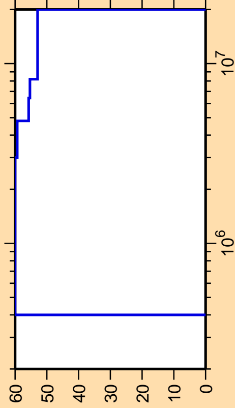
\Delta\sigma/\sigma vs. E for ^{87}\text{Mo}(n,n_2)
