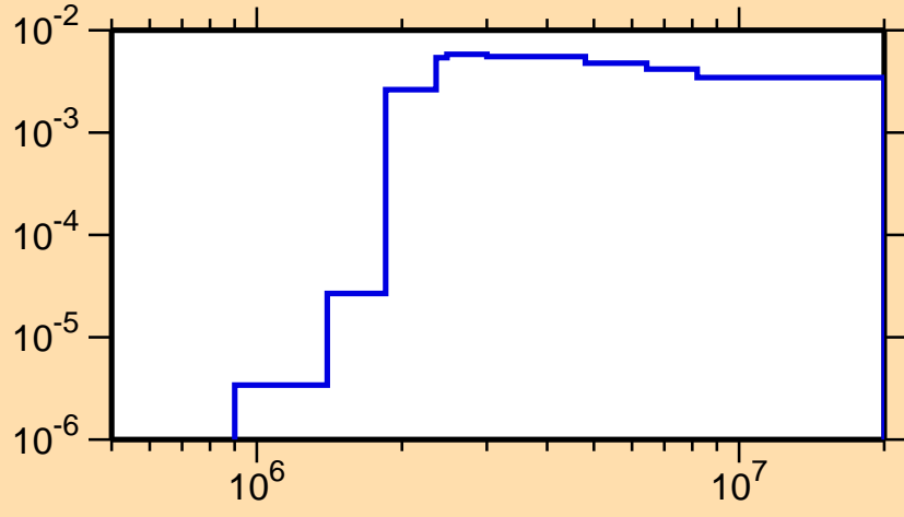
\sigma vs. E for ^{87}\text{Mo}(n,n\text{cont.})
