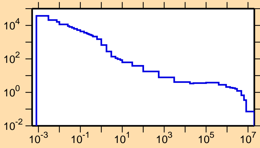
\sigma vs. E for ^{87}\text{Mo}(n,p)
