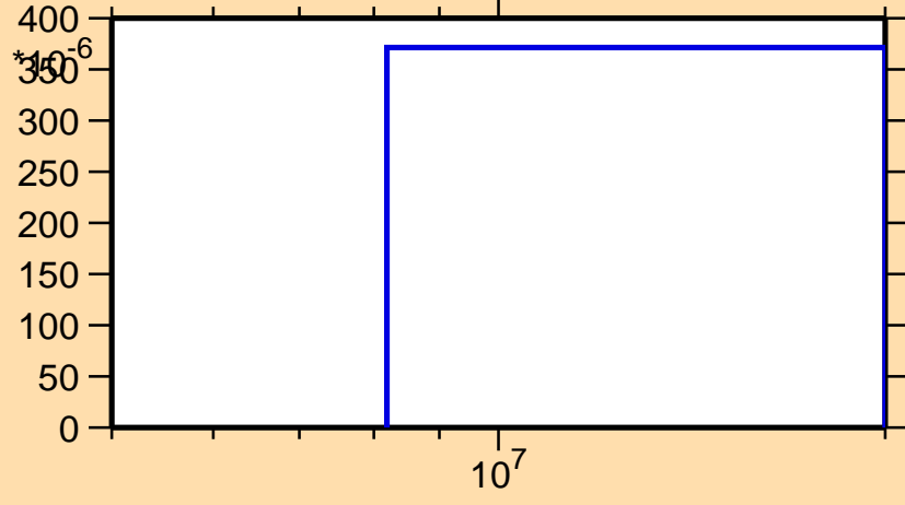
\sigma vs. E for ^{87}\text{Mo}(n,\text{pd})
