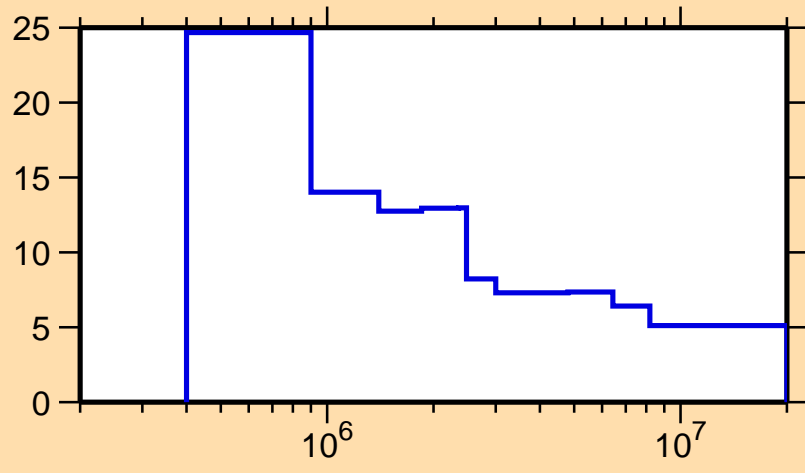
\Delta\sigma/\sigma vs. E for ^{87}\text{Mo}(n,n\text{onel.})
