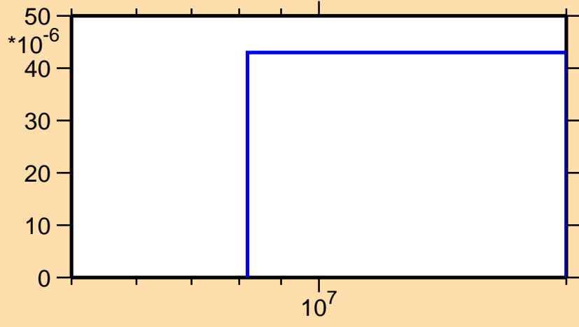
\sigma vs. E for ^{87}\text{Mo}(n,t)
