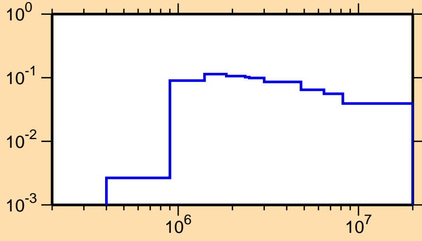
\sigma vs. E for ^{87}\text{Mo}(n,n_2)
