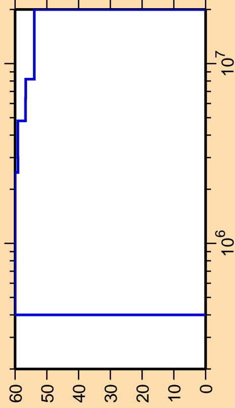
\Delta\sigma/\sigma vs. E for ^{87}\text{Mo}(n,n_3)
