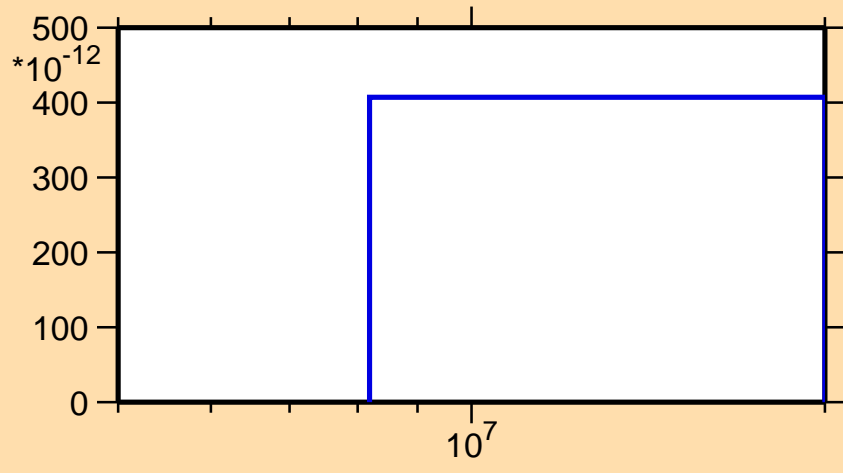
\sigma vs. E for ^{87}\text{Mo} (mt 34)
